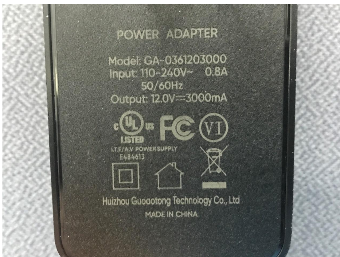
Photo 9 Appearance of adapter
