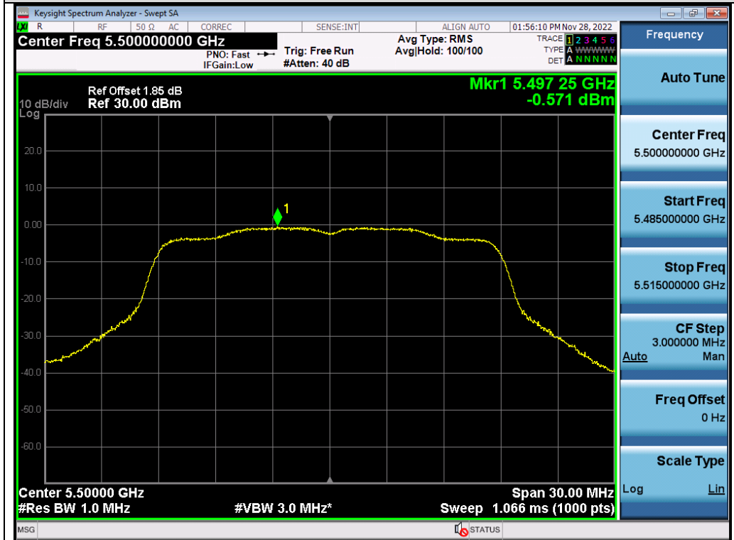
Test_Graph_802.11n20_ANT1_5500_MCS0_PSD
