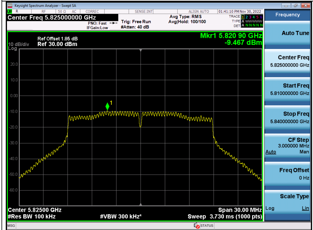
Test_Graph_802.11n20_ANT2_5825_MCS0_PSD
