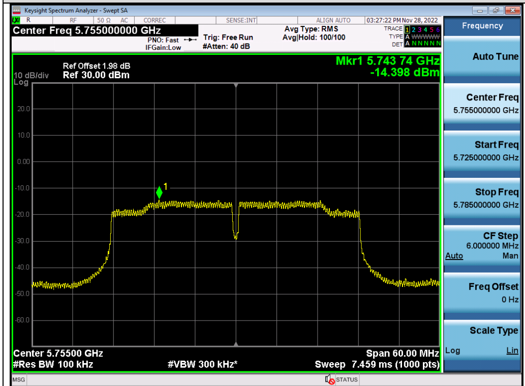
Test_Graph_802.11ac40_ANT1_5755_MCS9_PSD
