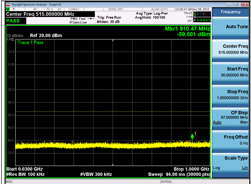
Test_Graph_802.11a_ANT1_5700_6Mbps_Frequency Band 1
