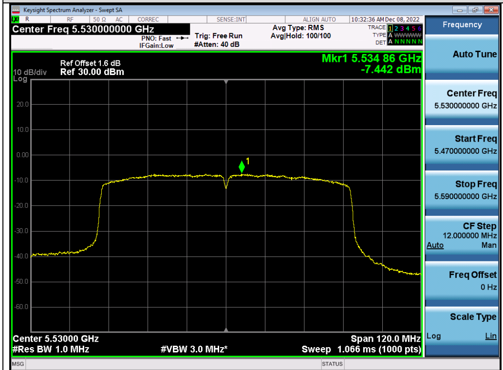
Test_Graph_802.11ac80_ANT1_5530_MCS9_PSD
