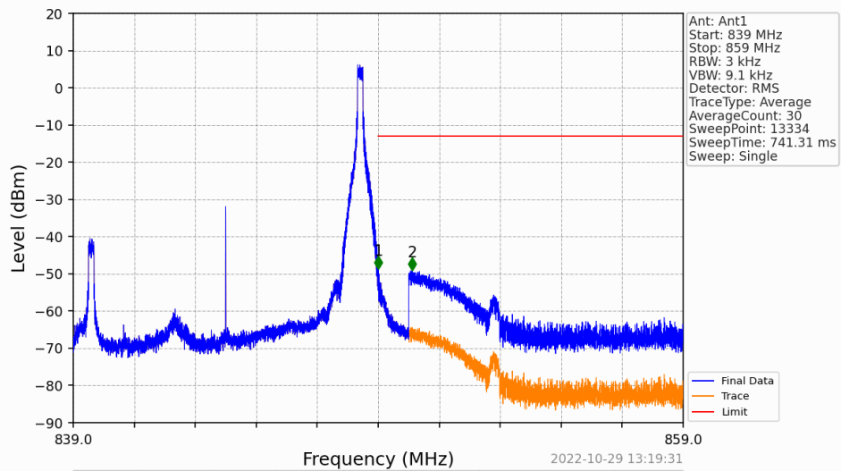
Band5_10MHz_16QAM_HCH_844MHz_RB_1_49_NTNV
