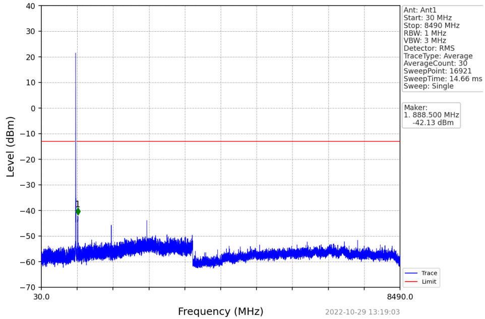
Band5_10MHz_16QAM_HCH_844MHz_RB_1_49_NTNV
