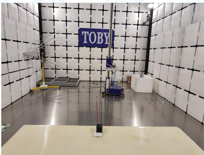
Radiated Emission Test Setup(30MHz-1GHz) Battery mode: EUT+Load
