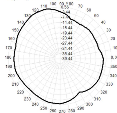
Total(H-XY), Max= 0.56dBi, CirD=10.12
