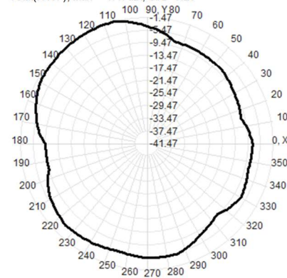
Total(H-XY), Max= -1.47dBi, CirD=9.29
