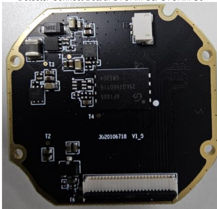
Detector Connect Board: STORM S3/ STORM S6
