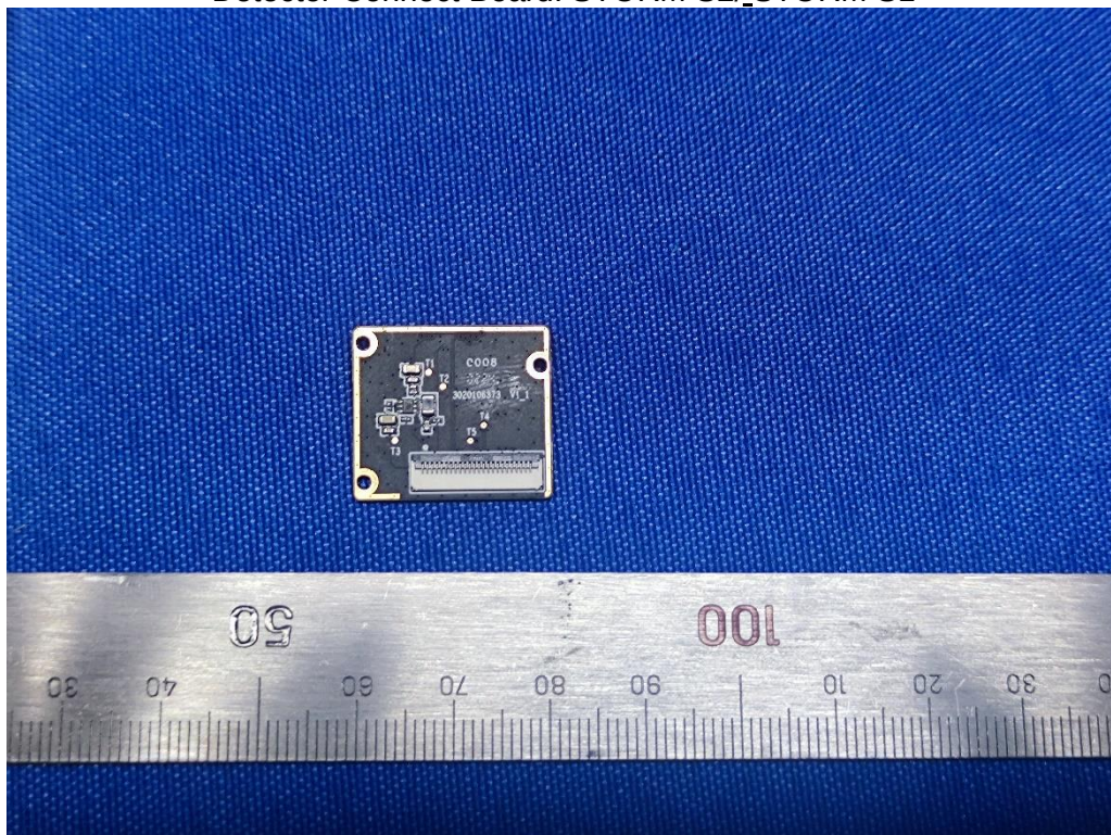
Detector Connect Board: STORM S2/_STORM S1
