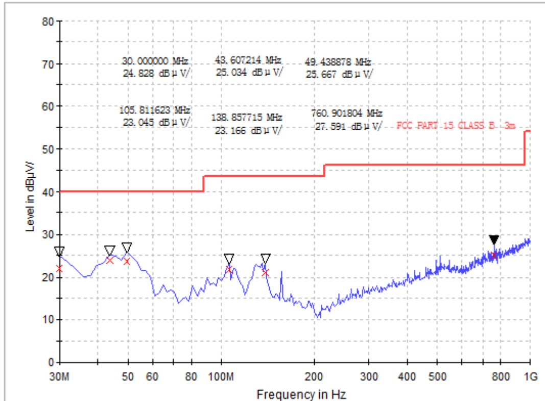
EMI Sweep-3M(30-1G)
