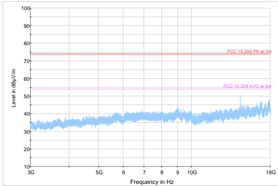
Plot # 18. Radiated Emissions: 3-18 GHz
