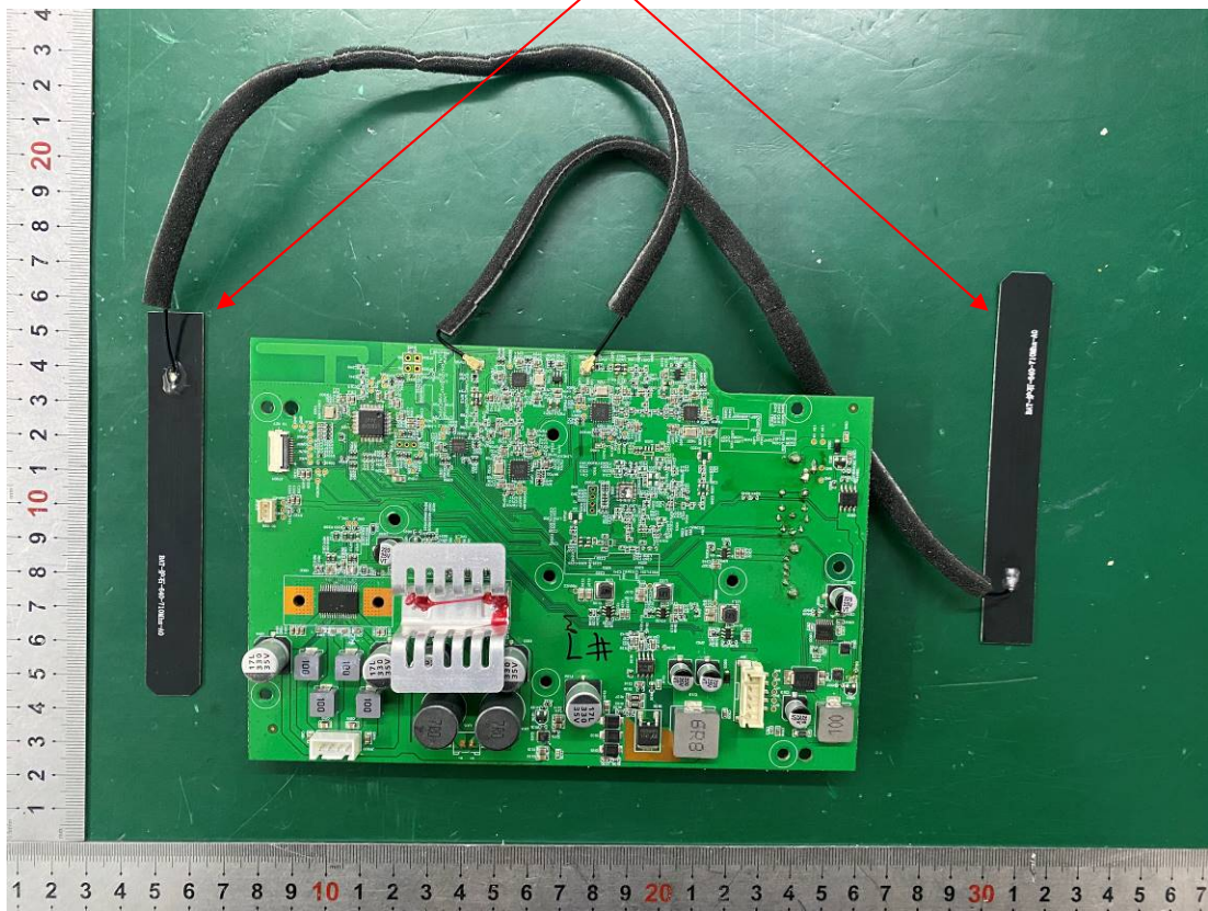
Microphone Receiving Antenna
