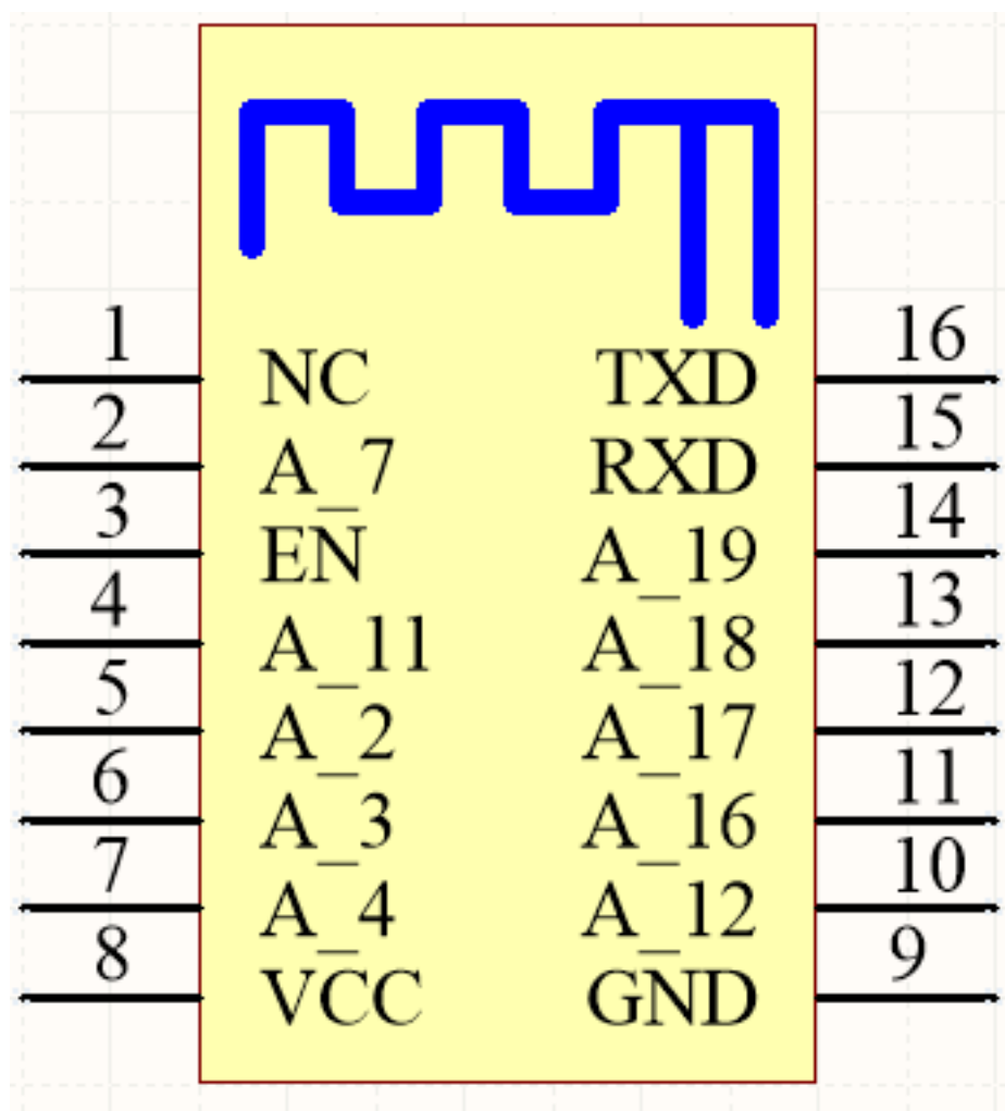
WBR3 PCB 封装
