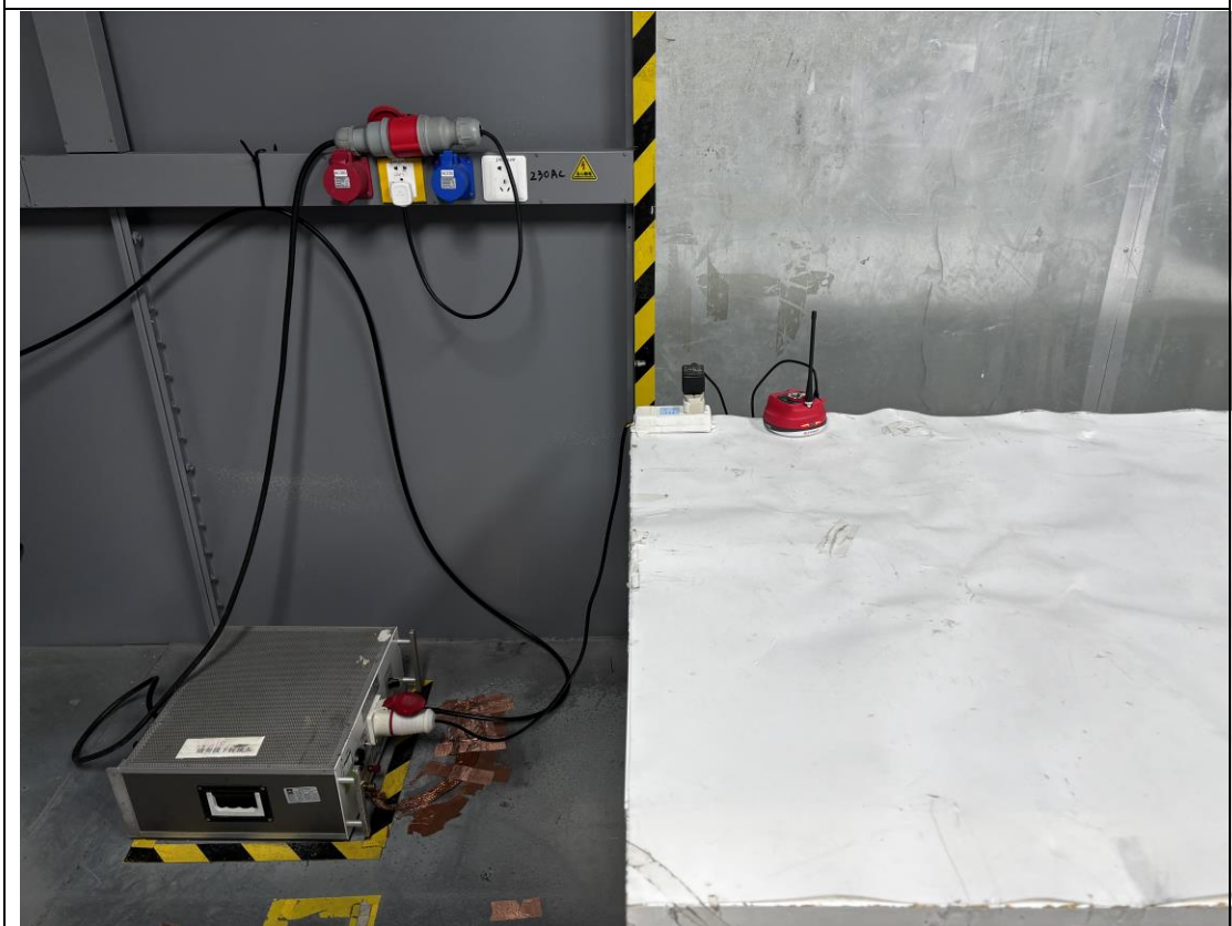
Conducted emission
