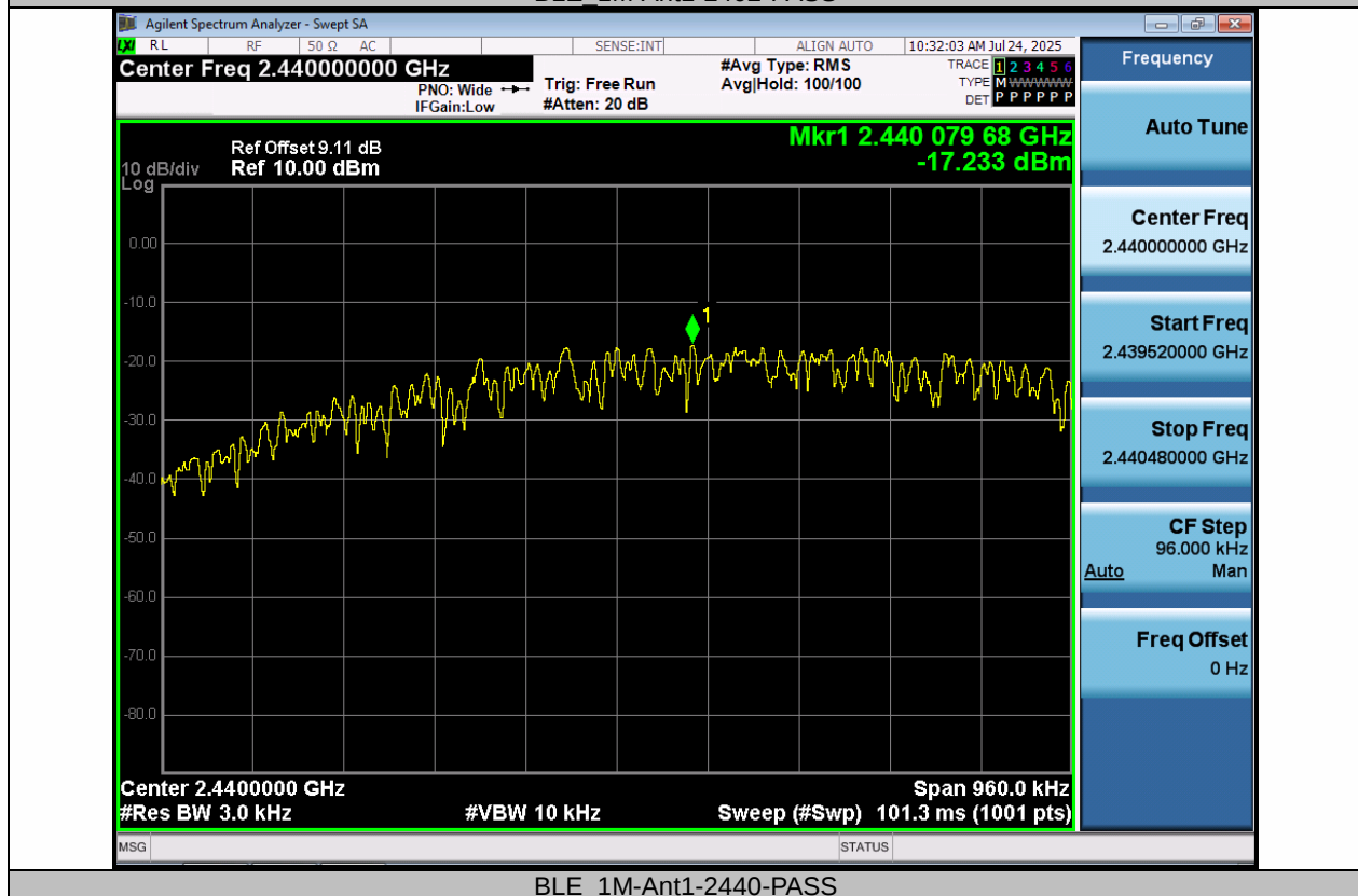
BLE_1M-Ant1-2440-PASS
