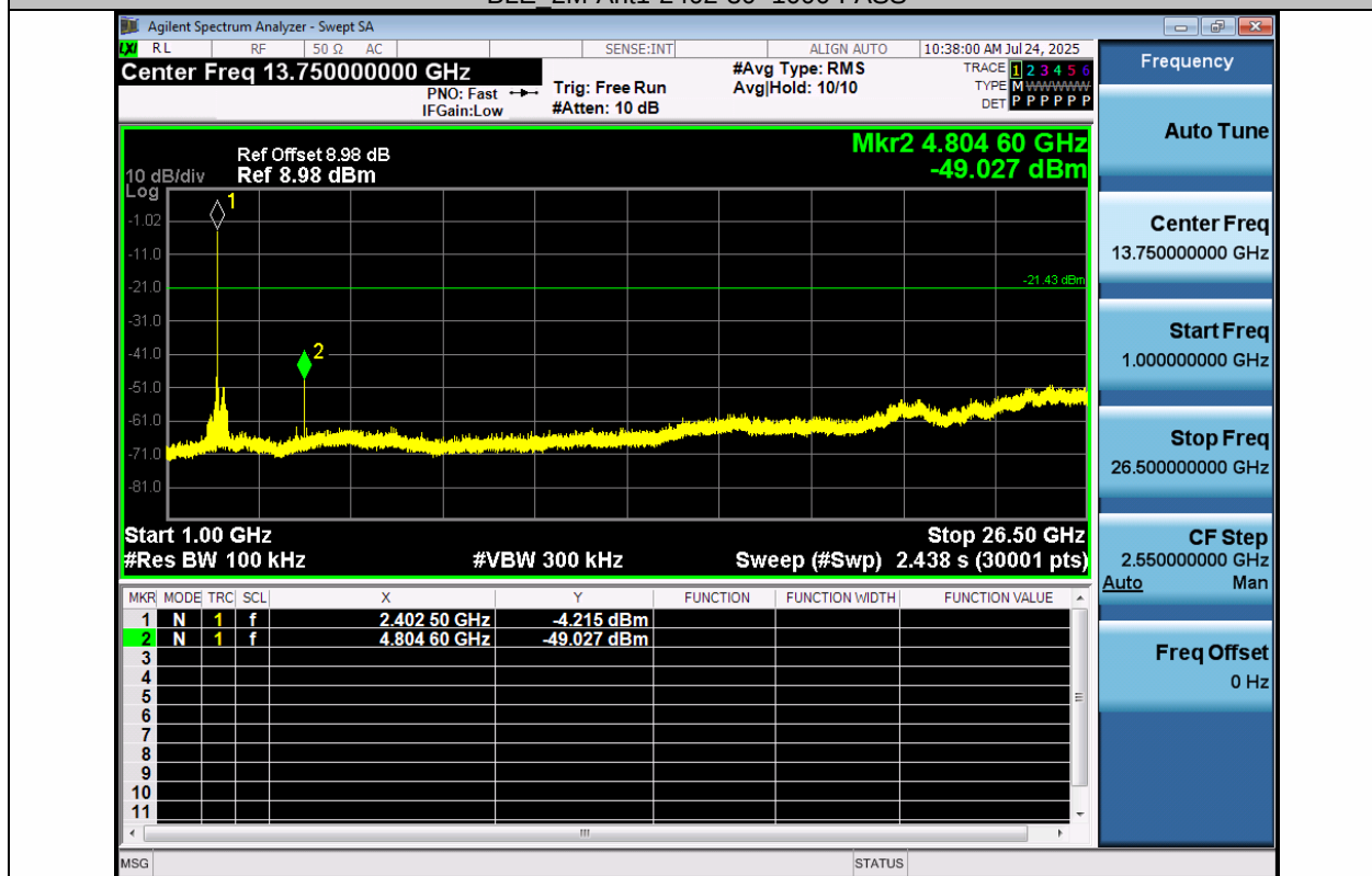
BLE_2M-Ant1-2402-1000~26500-PASS
