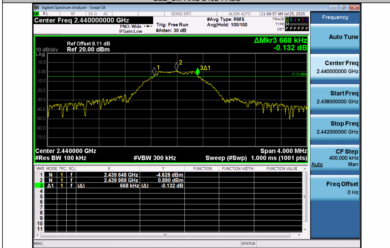
BLE_1M-Ant1-2440-PASS
