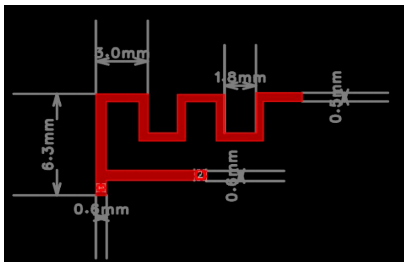
Nano Dongle PIFA Antenna
