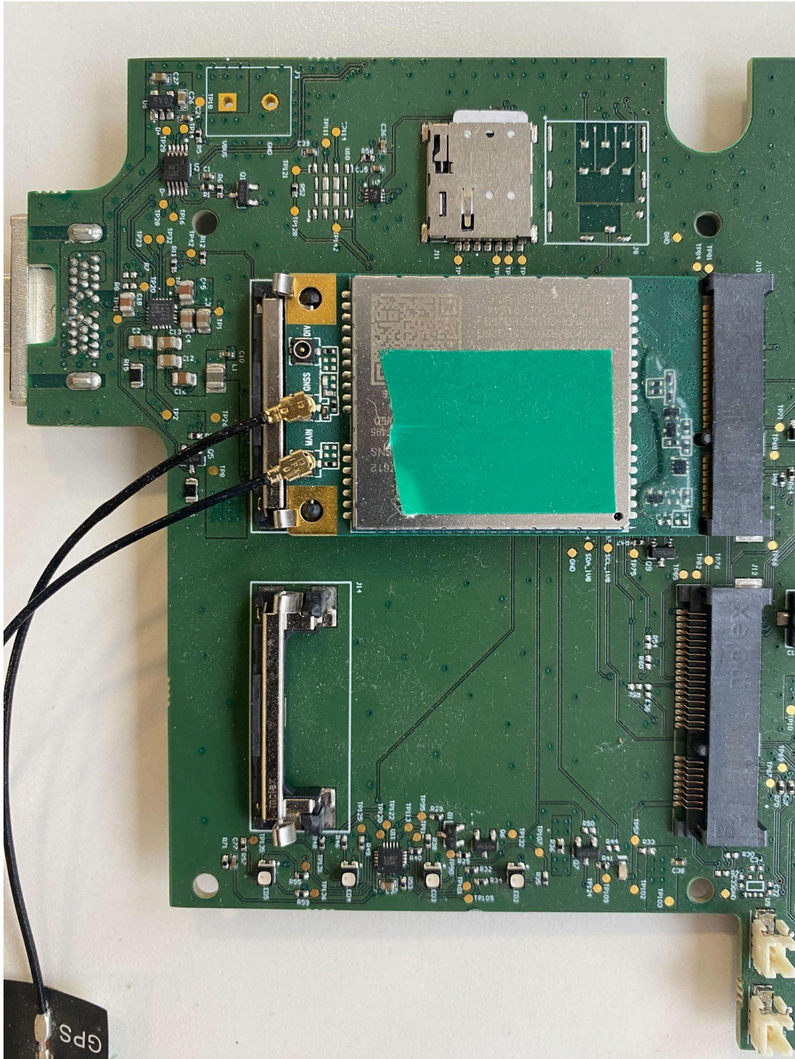
PCB Top View Zoomed In Lower Half
