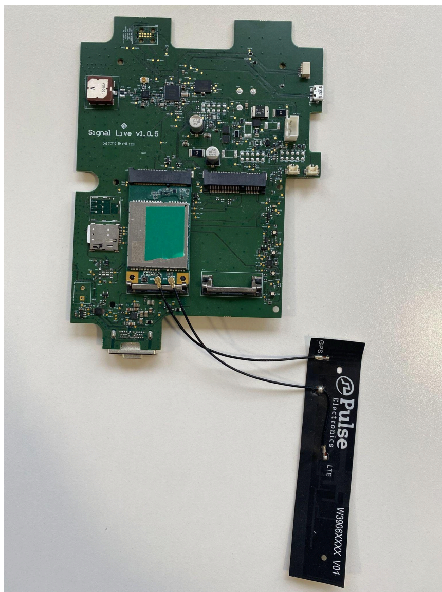
PCB Top View
