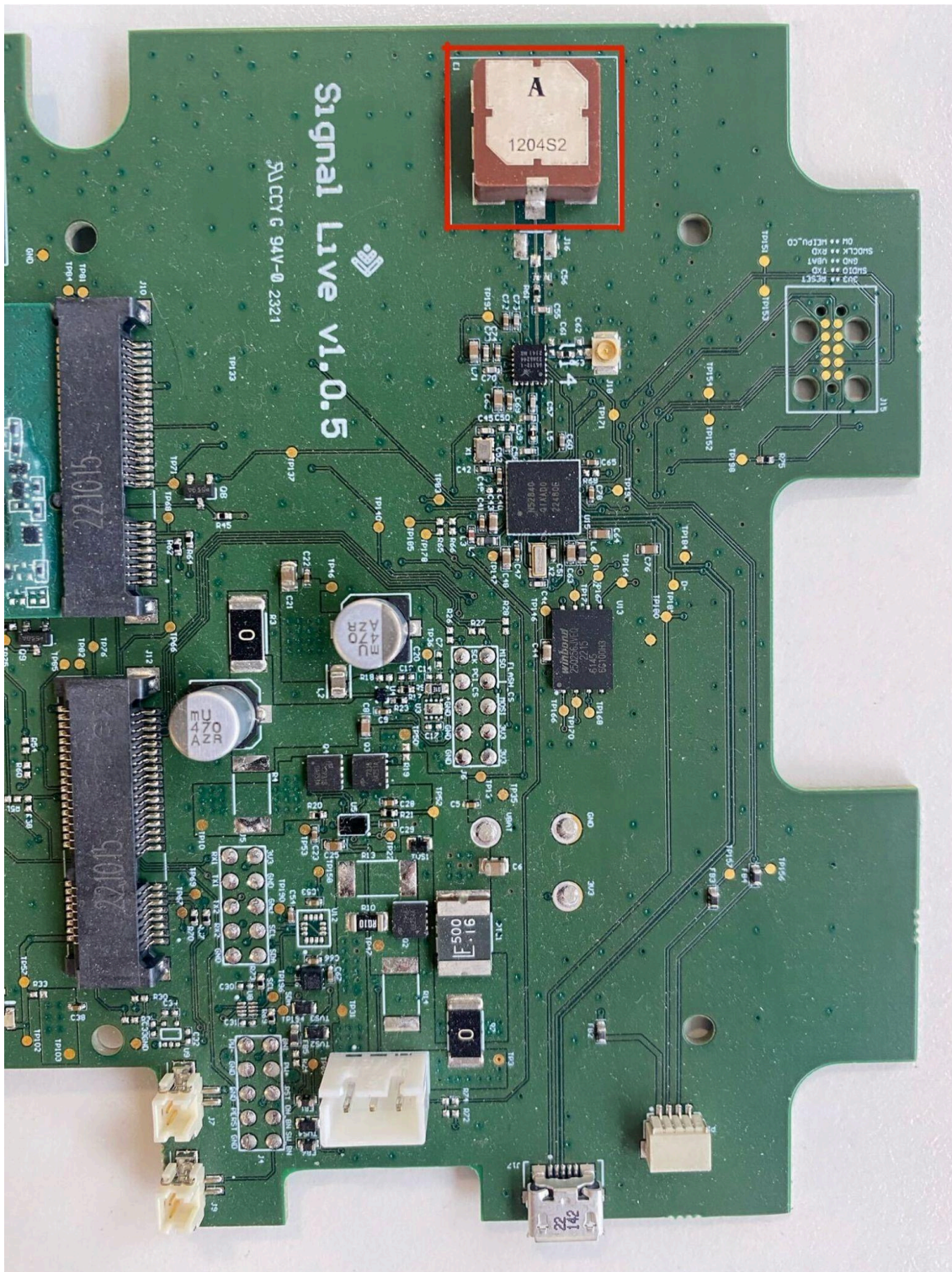
PCB Top View Zoomed In Upper Half (with Bluetooth LE Antenna indicated in red)
