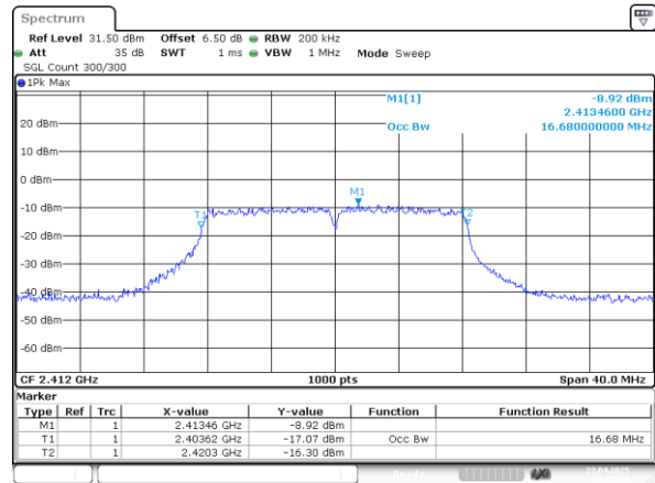
802.11g_2412MHz
