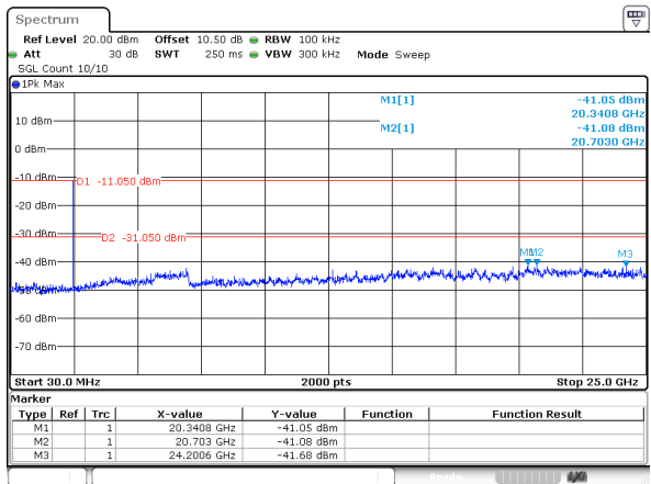
802.11g_2472MHz
