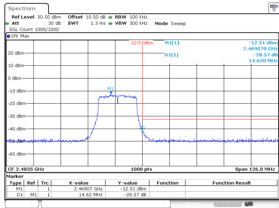
802.11n20_2472MHz
