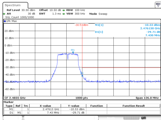
802.11g_2472MHz
