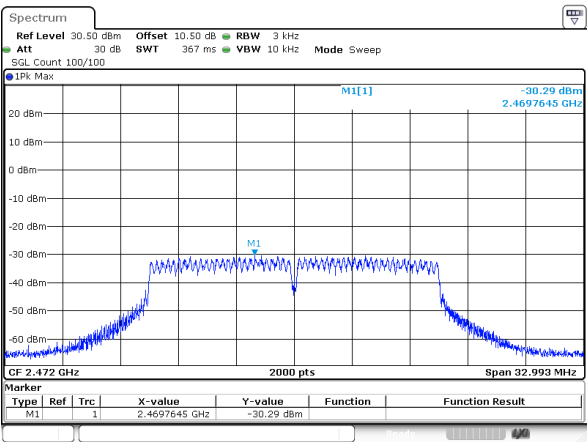
802.11g_2472MHz
