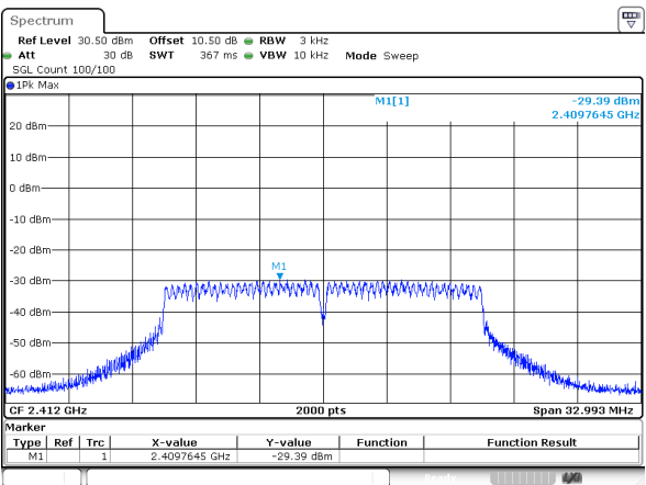
802.11g_2412MHz
