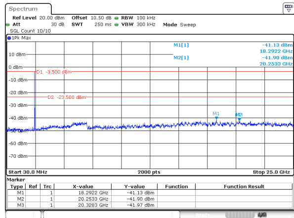
802.11g_2442MHz
