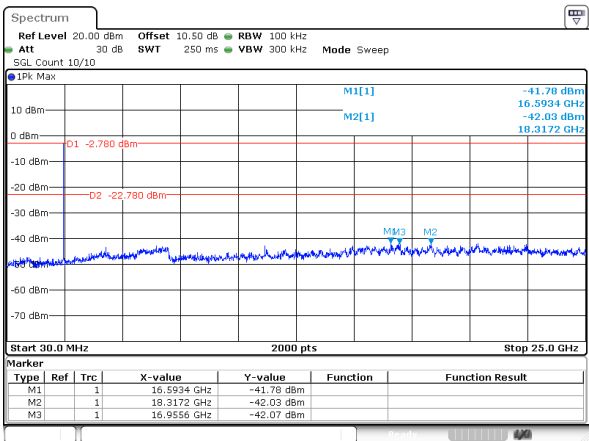
802.11g_2472MHz
