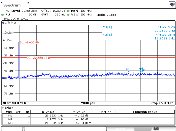
802.11g_2412MHz
