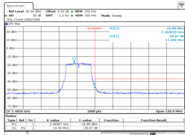
802.11n20_2472MHz
