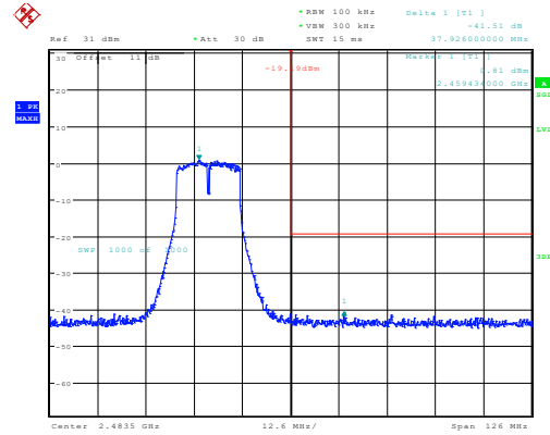
802.11g_2462MHz 41.51dB
