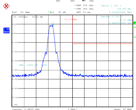
BLE_1M_High_Channel
