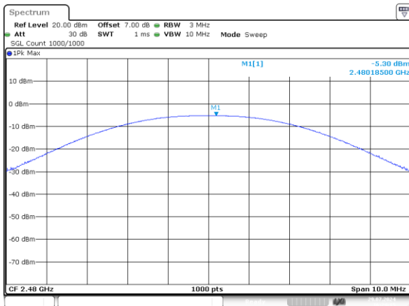
High -5.30dBm
