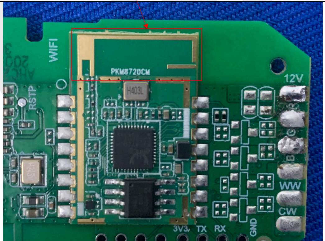
2.4G WiFi ANT
