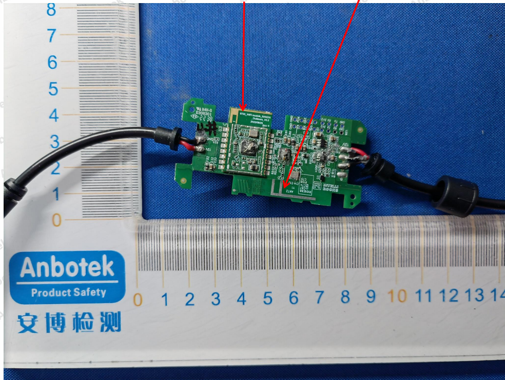
Internal Photograph WIFI ANT BT ANT
