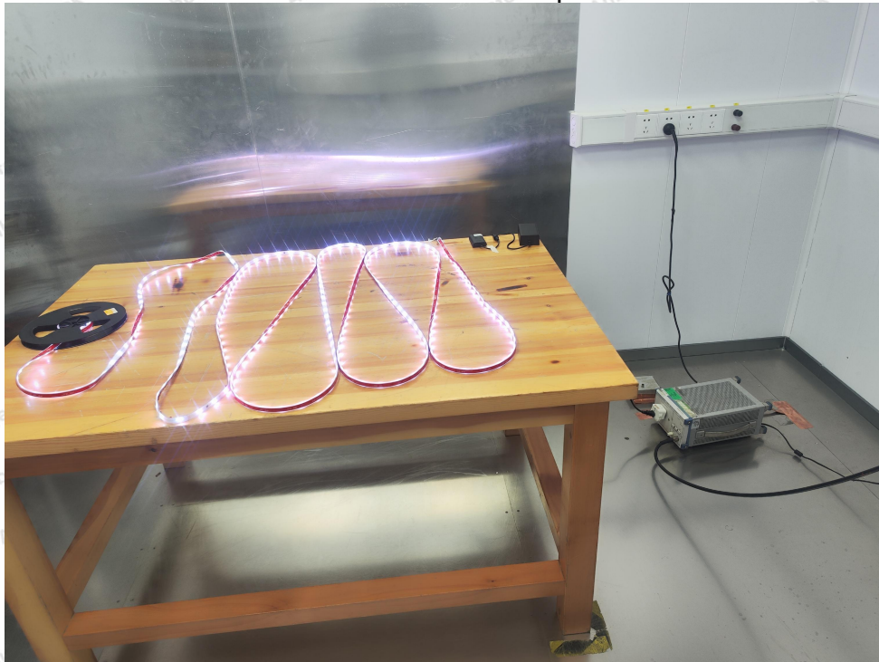
Model: H616C Conducted Emission at AC power line
