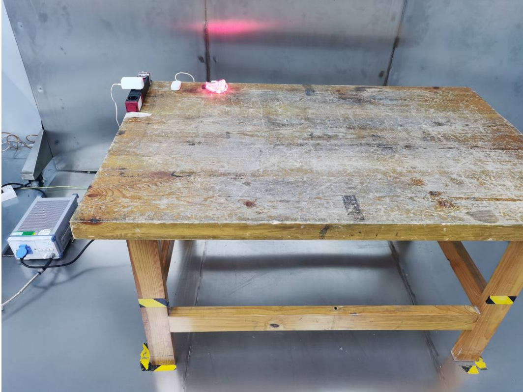
Conducted Emissions Side View (H6159)
