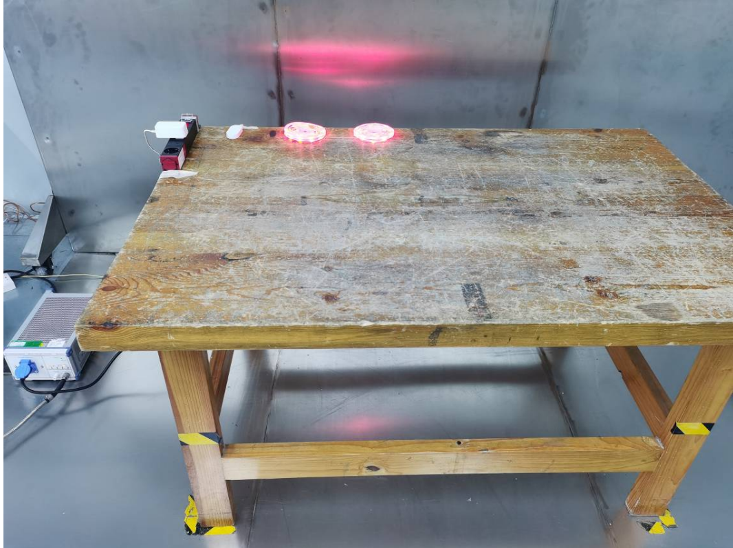
Conducted Emissions Side View (H614B)
