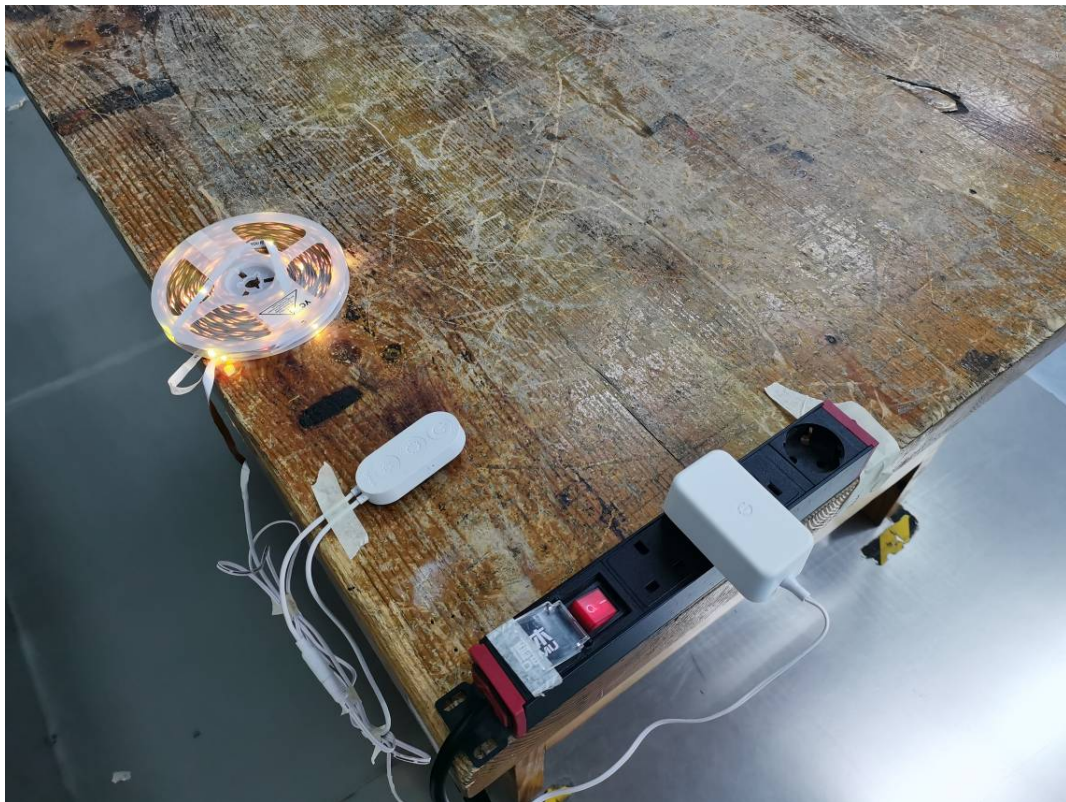
Conducted Emissions Side View (H615E)
