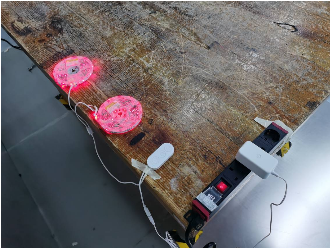
Conducted Emissions Side View (H614E)
