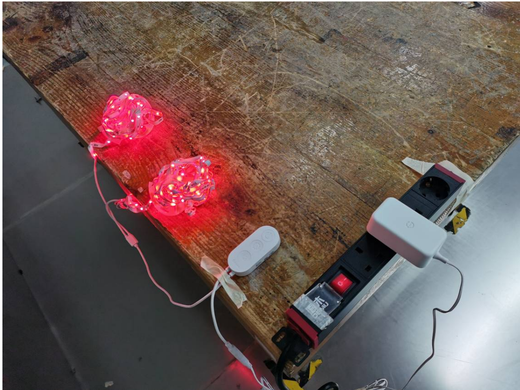
Conducted Emissions Side View (H6110)
