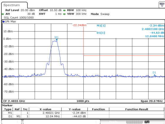
BLE_1M_High_Channel
