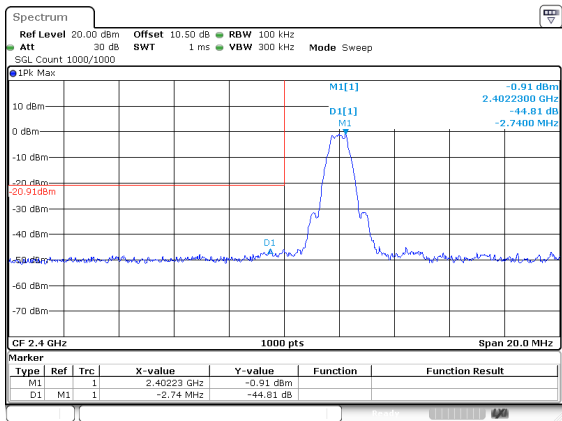
BLE_1M_Low_Channel
