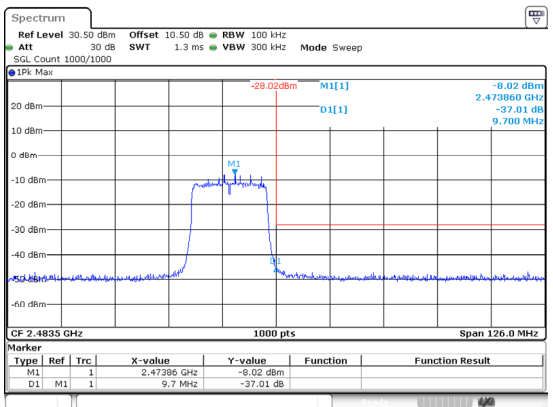
802.11n20_2472MHz
