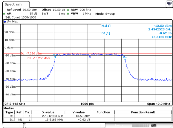
802.11g_2442MHz
