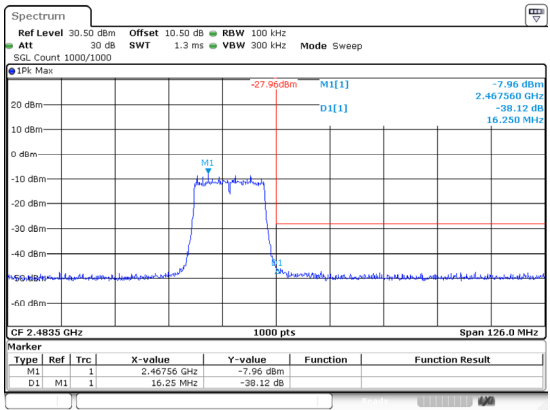
802.11g_2472MHz
