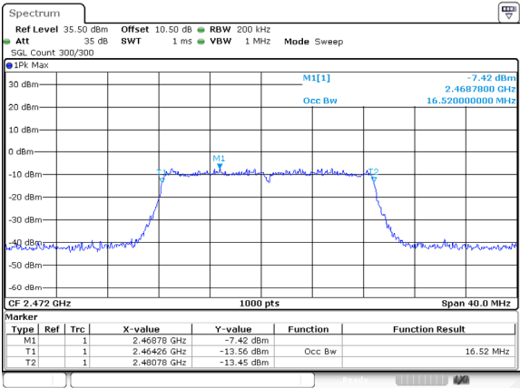
802.11g_2472MHz
