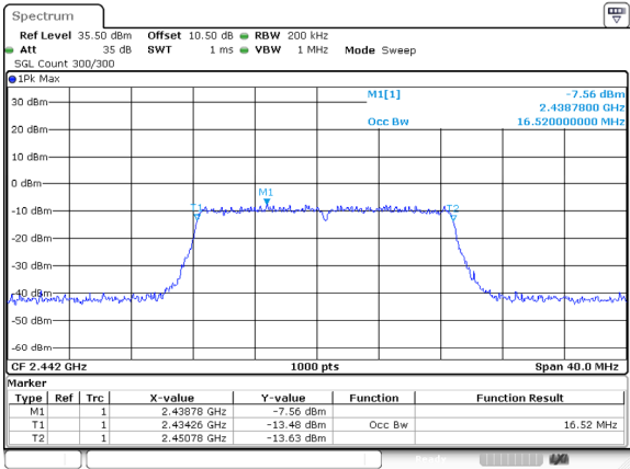
802.11g_2442MHz
