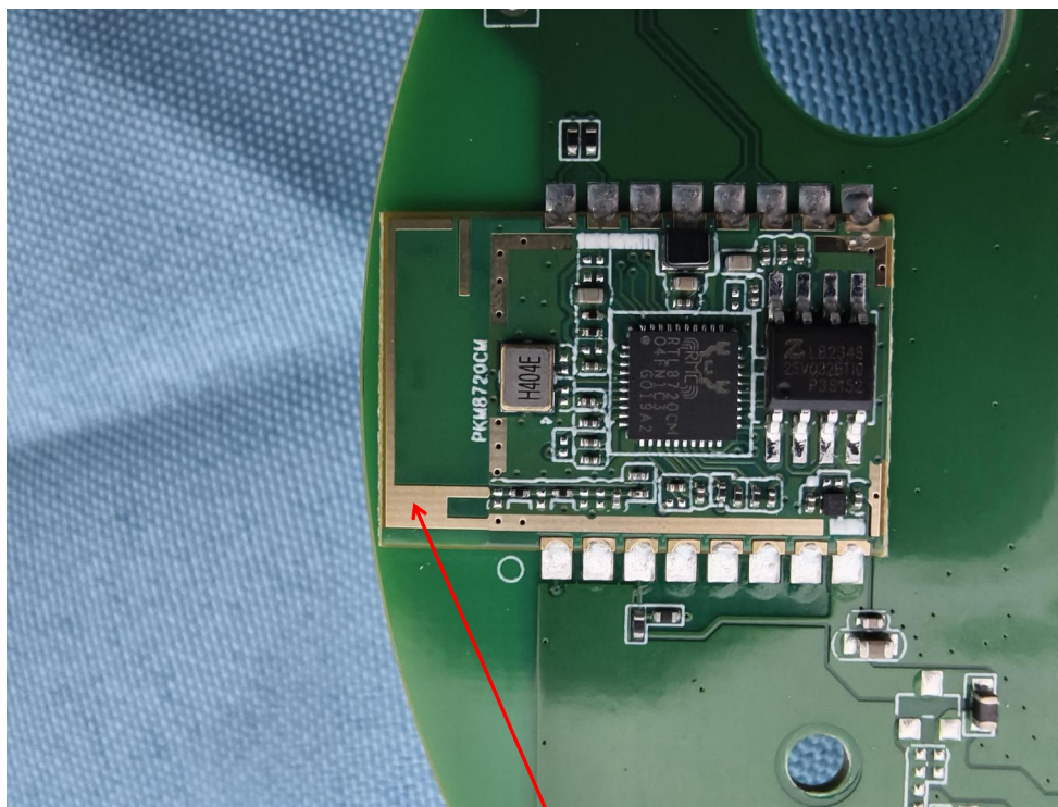
2.4G WiFi-ANT
