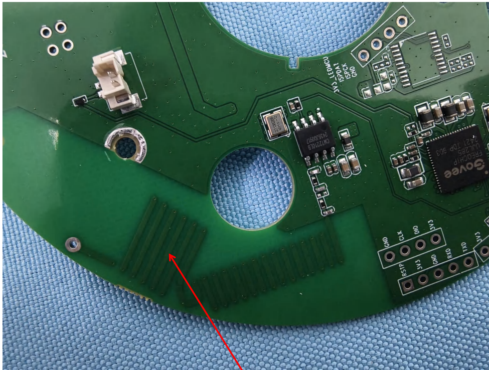
433.92MHz-RX-ANT
