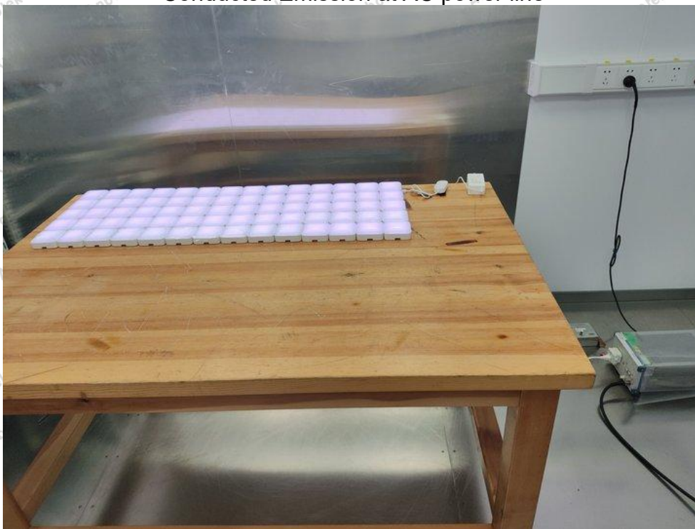
Model: H6069B(70PCS) Conducted Emission at AC power line
