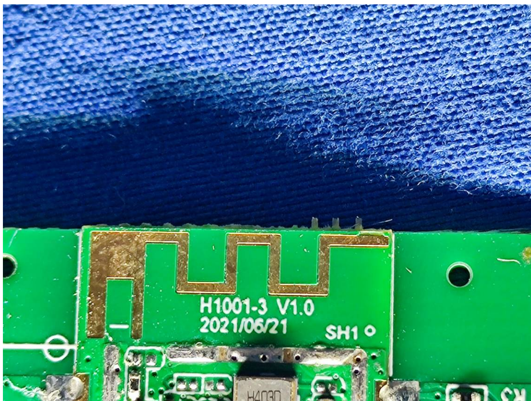
Buletooth&Wifi Antenna
