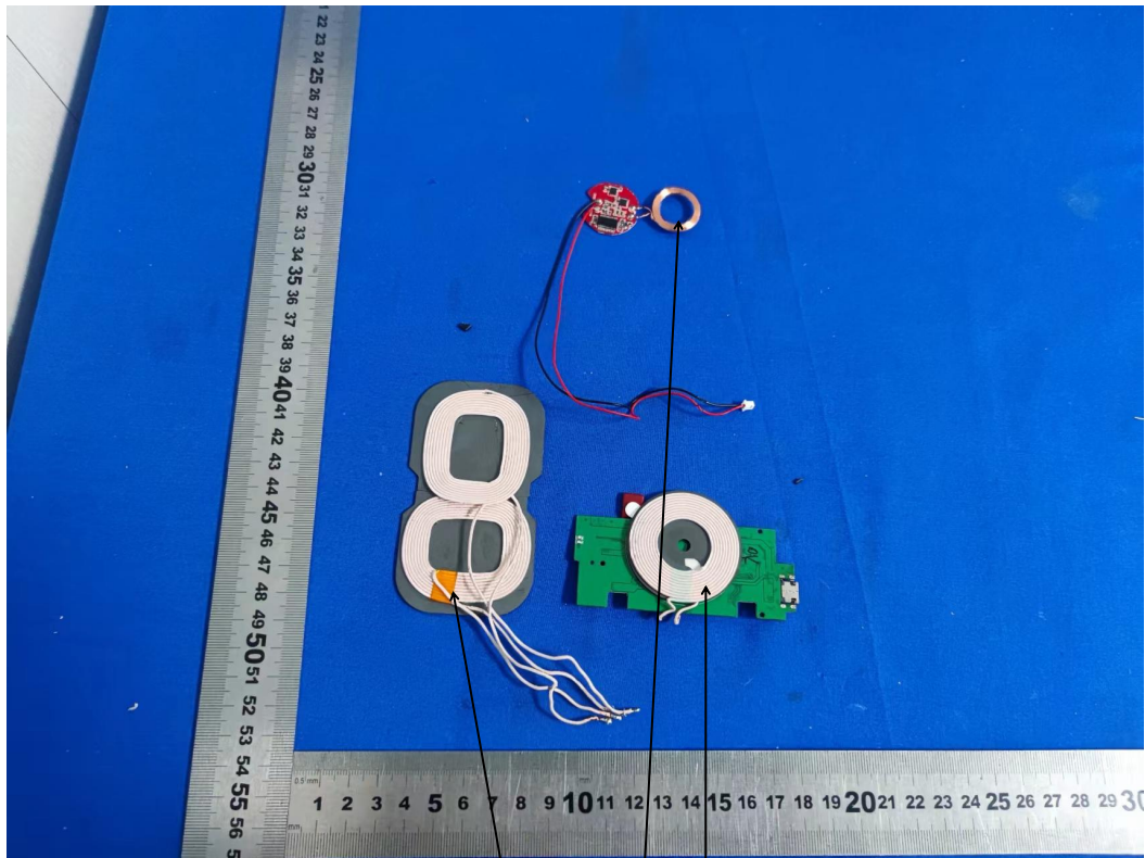
Inductive Loop Antenna
