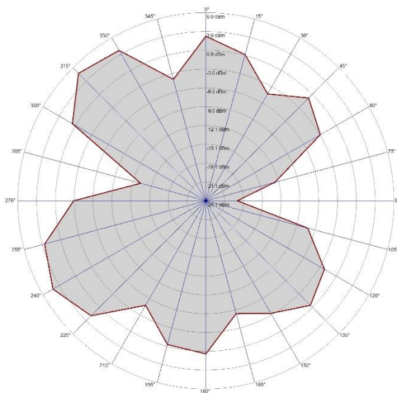
Figure 5 – 2426 MHz, Horizontal
