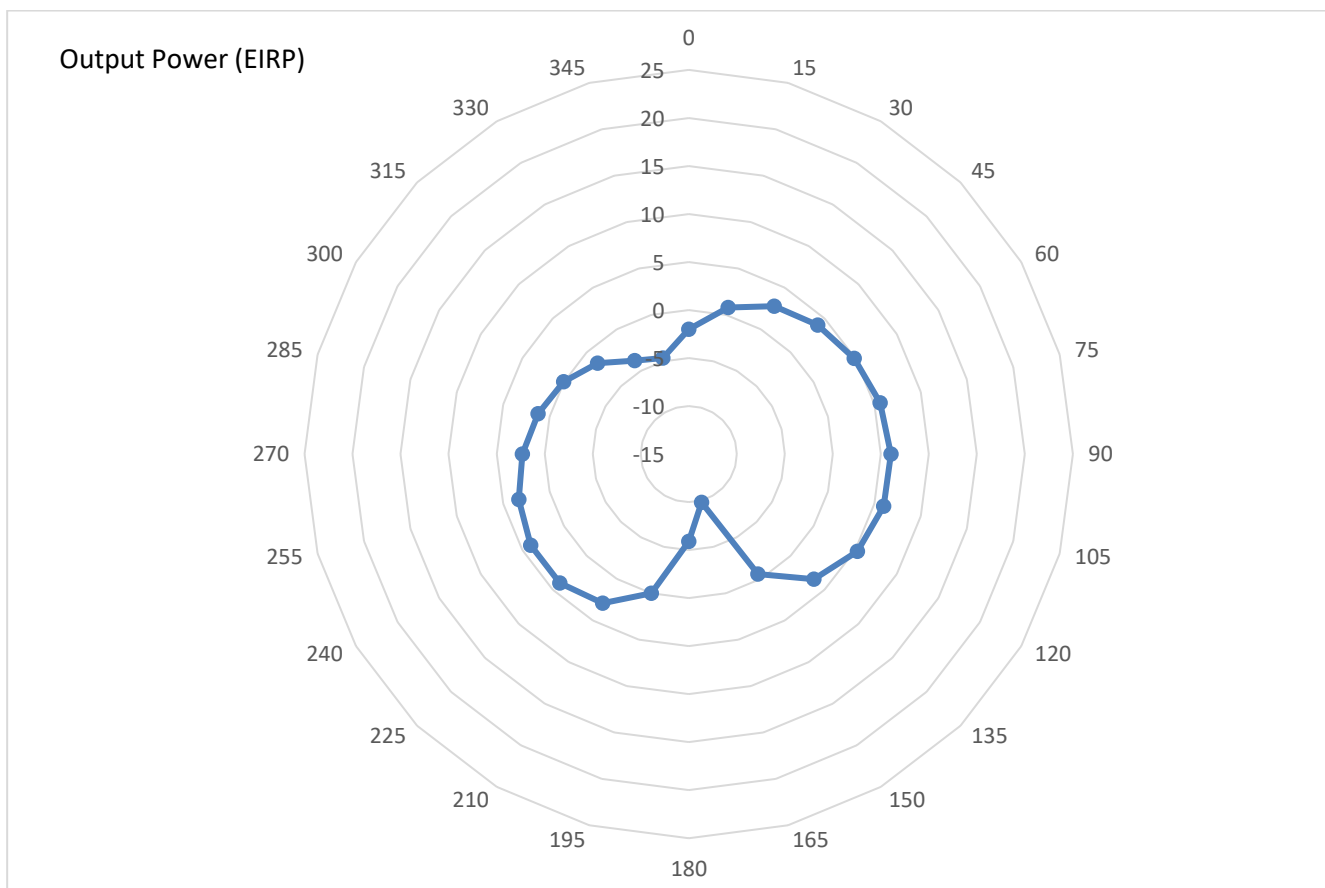
Figure 18 – 707.5 MHz, Vertical
