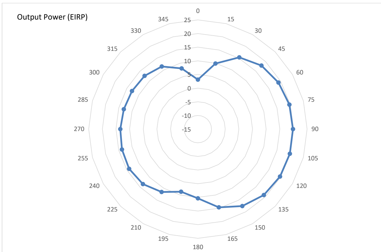
Figure 14 – 846.5 MHz, Vertical
