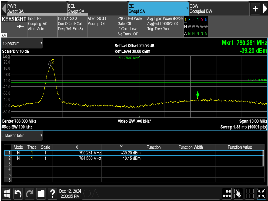
Figure 11 - Upper Band Edge, 784.5 MHz, Modulation: \pi/2 -BPSK, SCS: 3.75 kHz, Tone Number: 1, Start Sub-Carrier: 47
