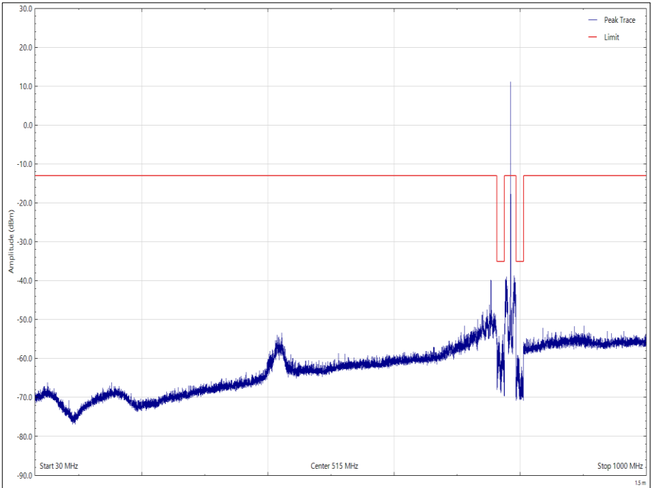
Figure 37 - 784.5 MHz - 30 MHz to 1 GHz, Vertical, Orientation Y, Top Channel
