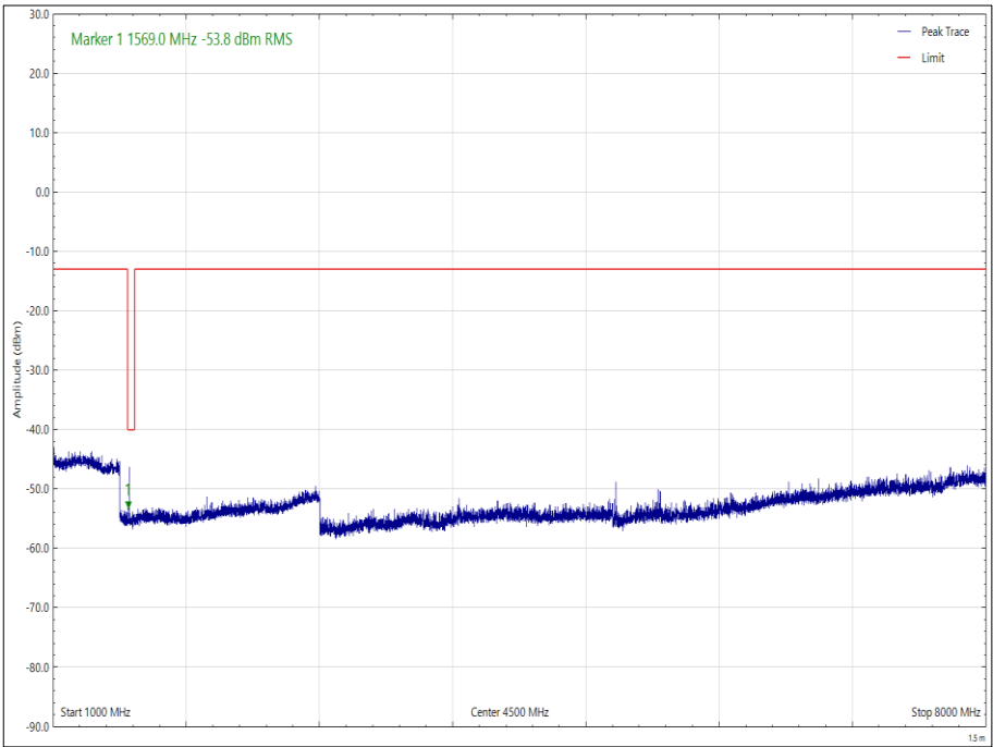
Figure 42 - 784.5 MHz - 1 GHz to 8 GHz, Vertical, Orientation Z, Top Channel
