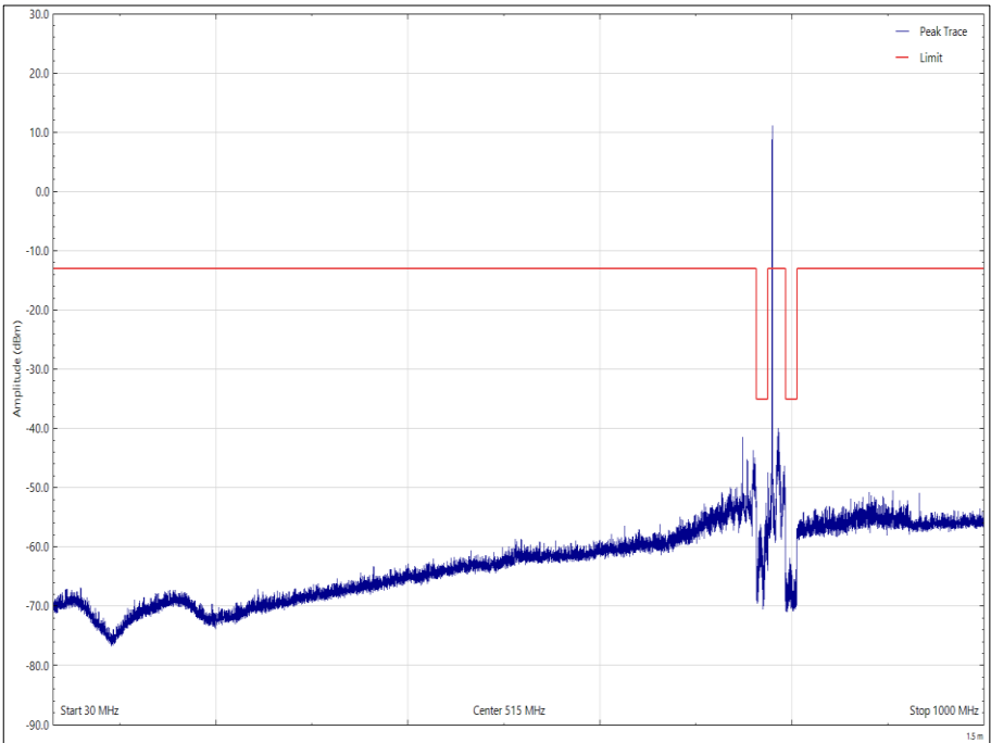
Figure 27 - 779.5 MHz - 30 MHz to 1 GHz, Horizontal, Orientation Z, Bottom Channel
