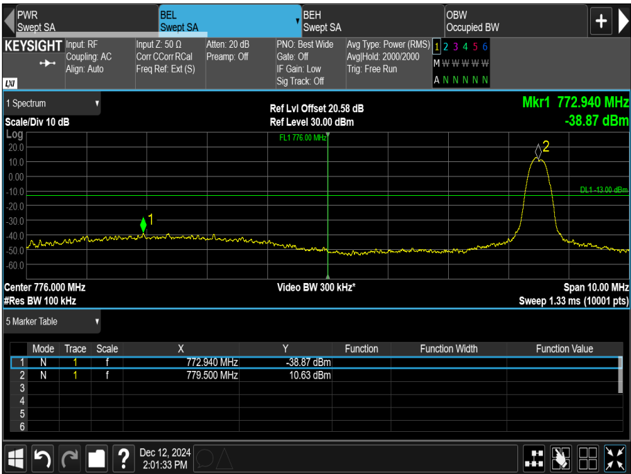
Figure 7 - Lower Band Edge, 779.5 MHz, Modulation: \pi/2 -BPSK, SCS: 3.75 kHz, Tone Number: 1, Start Sub-Carrier: 0
