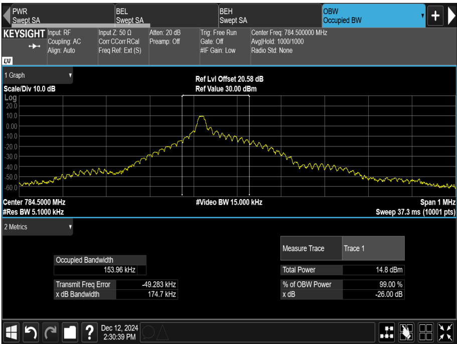
Figure 4 - Emission Bandwidth, 784.5 MHz, Modulation: \pi/2 -BPSK, SCS: 15 kHz, Tone Number: 1, Start Sub-Carrier: 0
