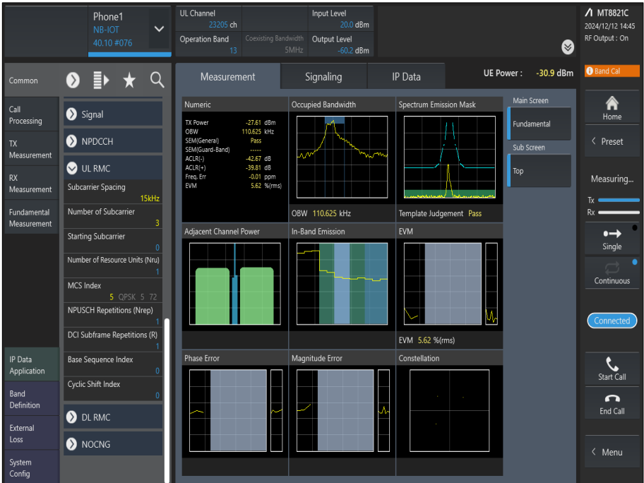
Figure 17 - QPSK MCS5
