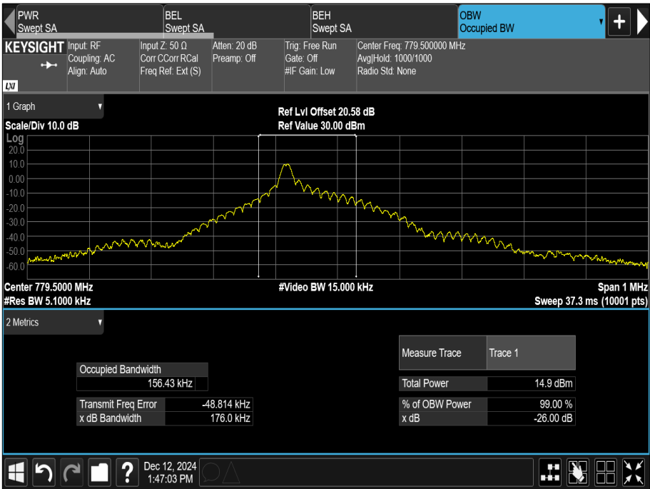
Figure 1 - Emission Bandwidth, 779.5 MHz, Modulation: \pi/2 -BPSK, SCS: 15 kHz, Tone Number: 1, Start Sub-Carrier: 0
