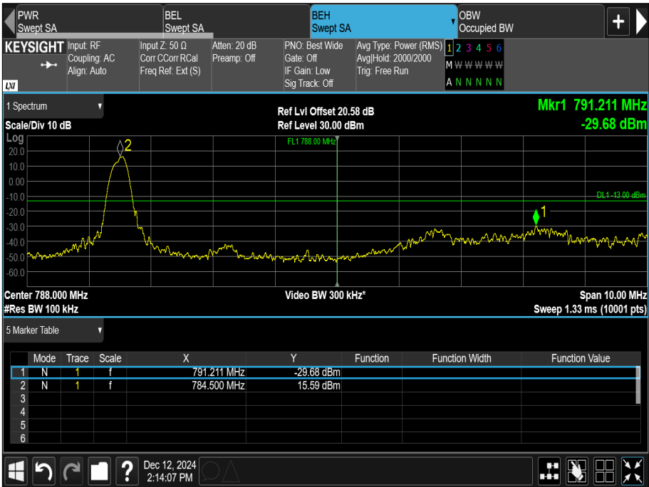
Figure 13 - Upper Band Edge, 784.5 MHz, Modulation: QPSK, SCS: 15 kHz, Tone Number: 3, Start Sub-Carrier: 6
