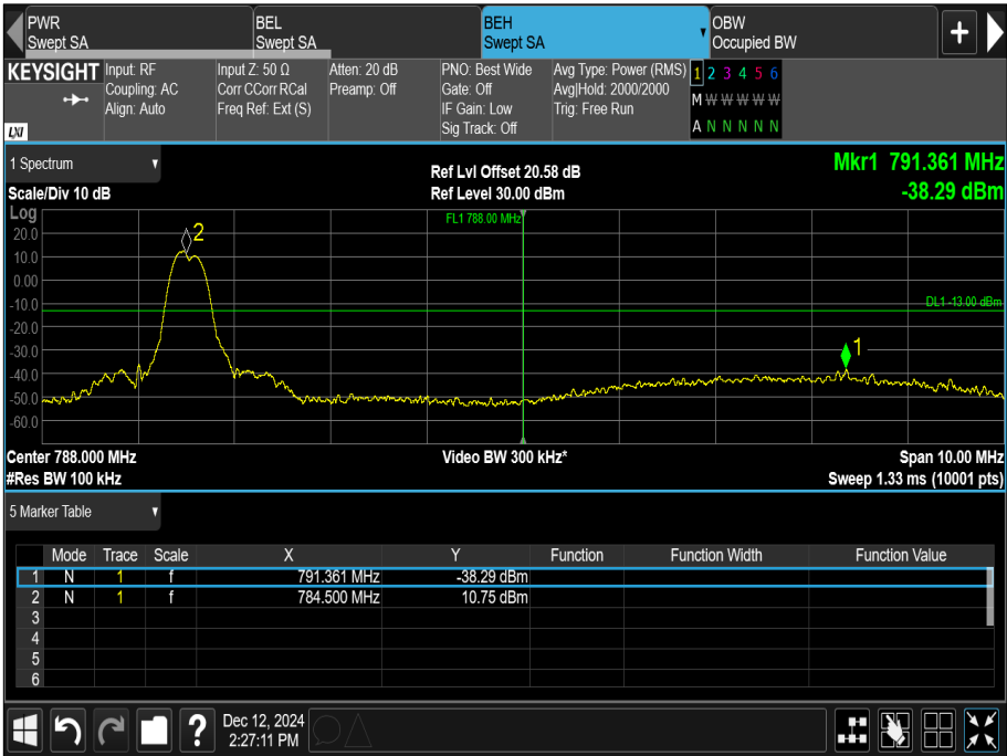
Figure 12 - Upper Band Edge, 784.5 MHz, Modulation: \pi/2 -BPSK, SCS: 15 kHz, Tone Number: 1, Start Sub-Carrier: 11
