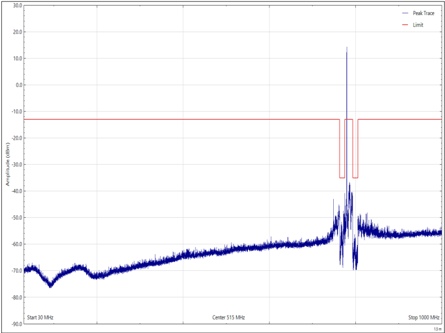
Figure 21 - 779.5 MHz - 30 MHz to 1 GHz, Vertical, Orientation X, Bottom Channel
