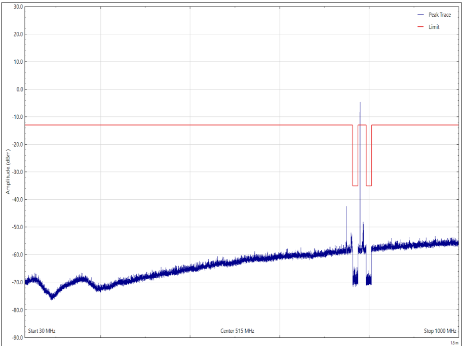
Figure 29 - 779.5 MHz - 30 MHz to 1 GHz, Vertical, Orientation Z, Bottom Channel
