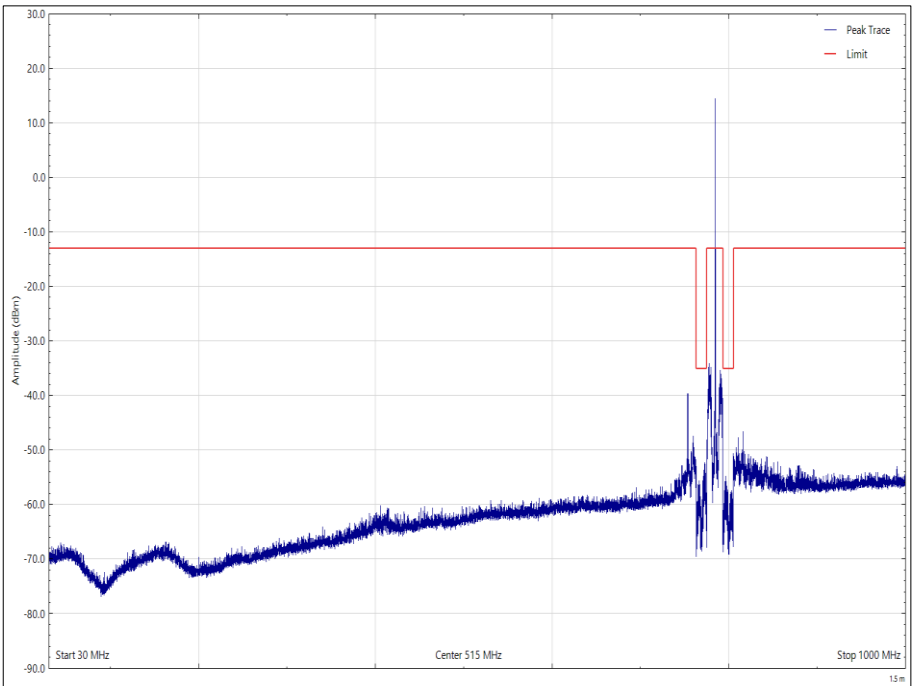
Figure 33 - 784.5 MHz - 30 MHz to 1 GHz, Vertical, Orientation X, Top Channel
