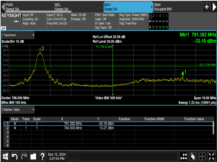
Figure 14 - Upper Band Edge, 784.5 MHz, Modulation: QPSK, SCS: 15 kHz, Tone Number: 12, Start Sub-Carrier: 0
