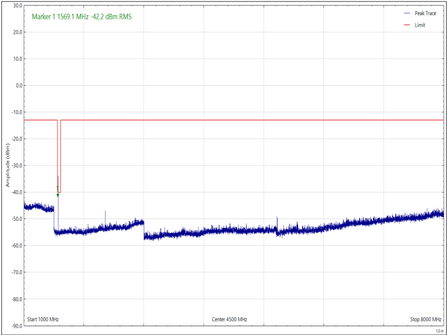
Figure 40 - 784.5 MHz - 1 GHz to 8 GHz, Horizontal, Orientation Z, Top Channel
