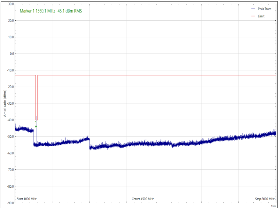
Figure 38 - 784.5 MHz - 1 GHz to 8 GHz, Vertical, Orientation Y, Top Channel
