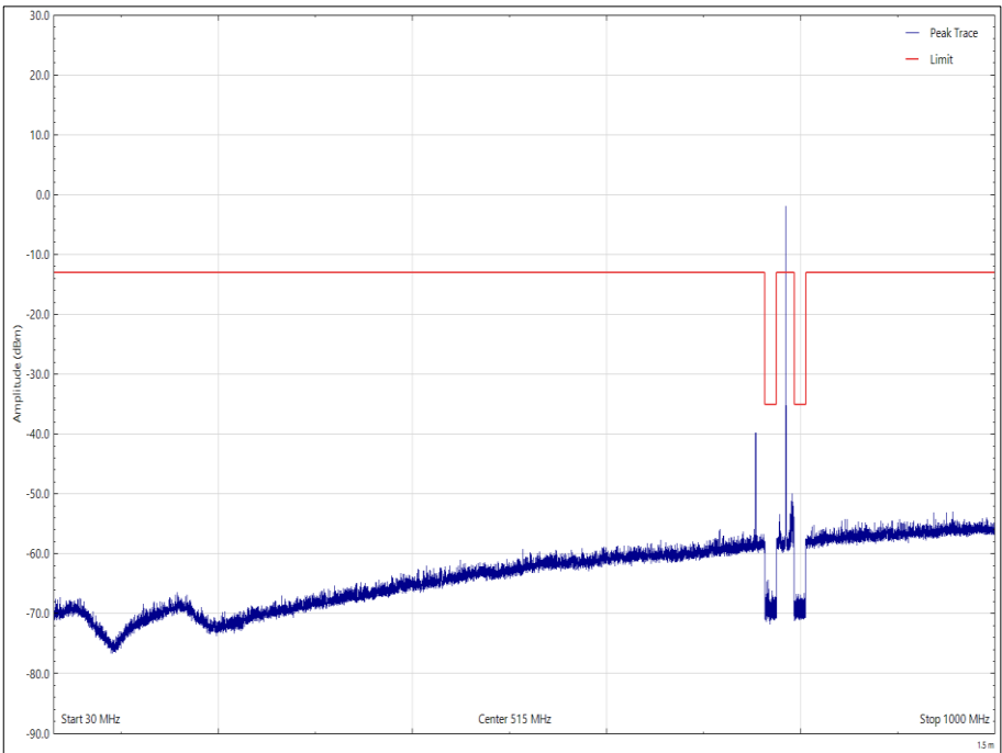
Figure 41 - 784.5 MHz - 30 MHz to 1 GHz, Vertical, Orientation Z, Top Channel
