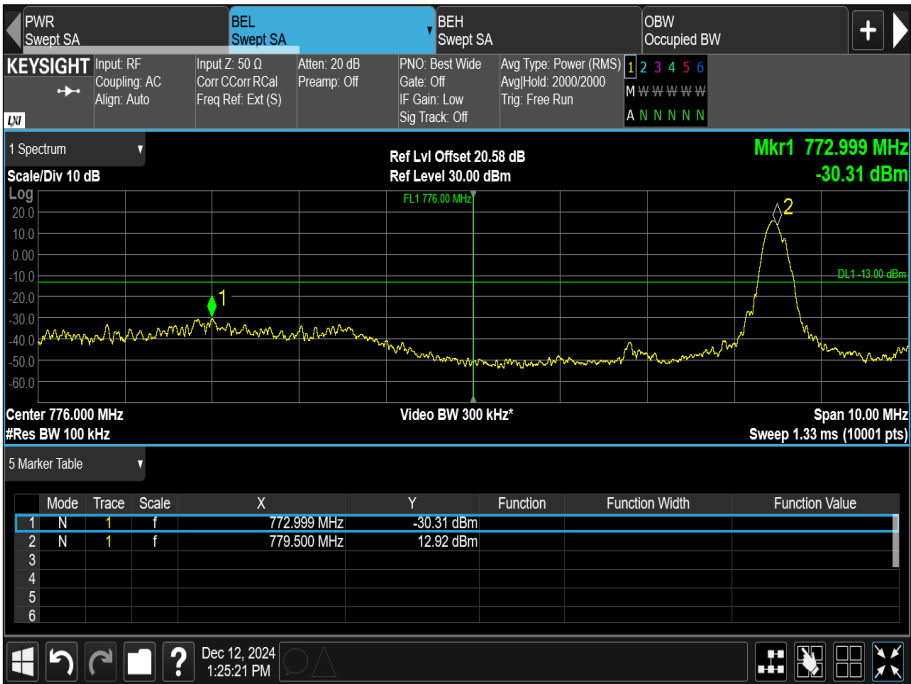
Figure 9 - Lower Band Edge, 779.5 MHz, Modulation: QPSK, SCS: 15 kHz, Tone Number: 3, Start Sub-Carrier: 0
