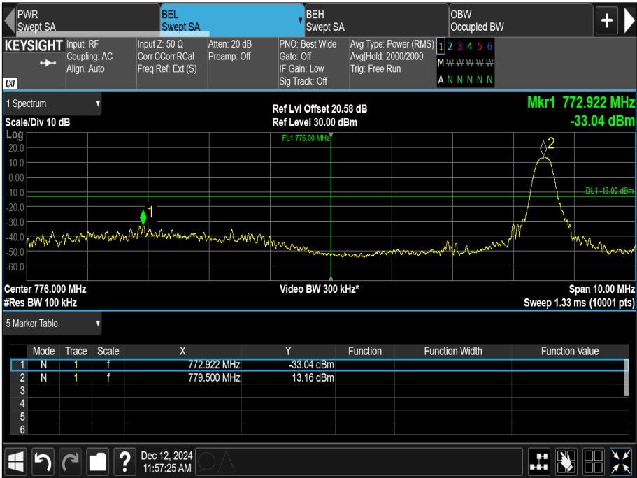
Figure 10 - Lower Band Edge, 779.5 MHz, Modulation: QPSK, SCS: 15 kHz, Tone Number: 12, Start Sub-Carrier: 0
