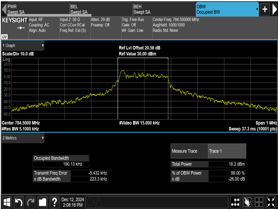
Figure 6 - Emission Bandwidth, 784.5 MHz, Modulation: QPSK, SCS: 15 kHz, Tone Number: 12, Start Sub-Carrier: 0
