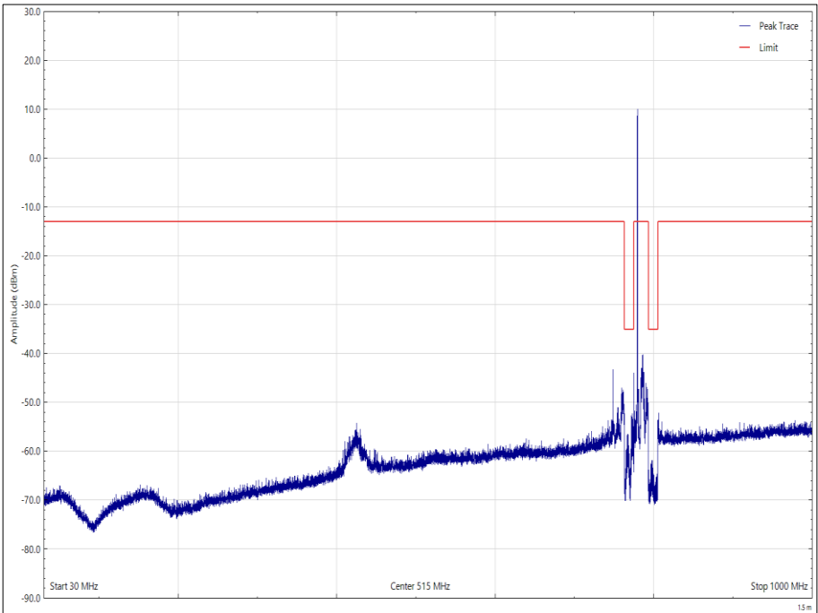
Figure 23 - 779.5 MHz - 30 MHz to 1 GHz, Horizontal, Orientation Y, Bottom Channel
