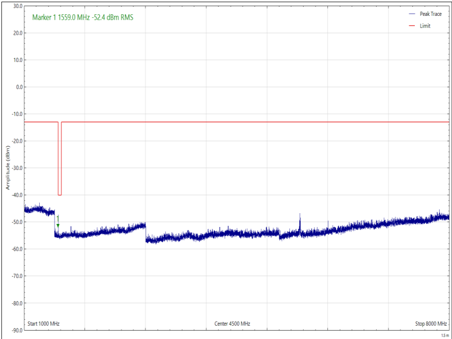
Figure 30 - 779.5 MHz - 1 GHz to 8 GHz, Vertical, Orientation Z, Bottom Channel
