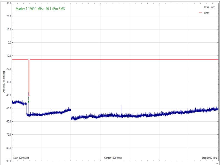
Figure 32 - 784.5 MHz - 1 GHz to 8 GHz, Horizontal, Orientation X, Top Channel
