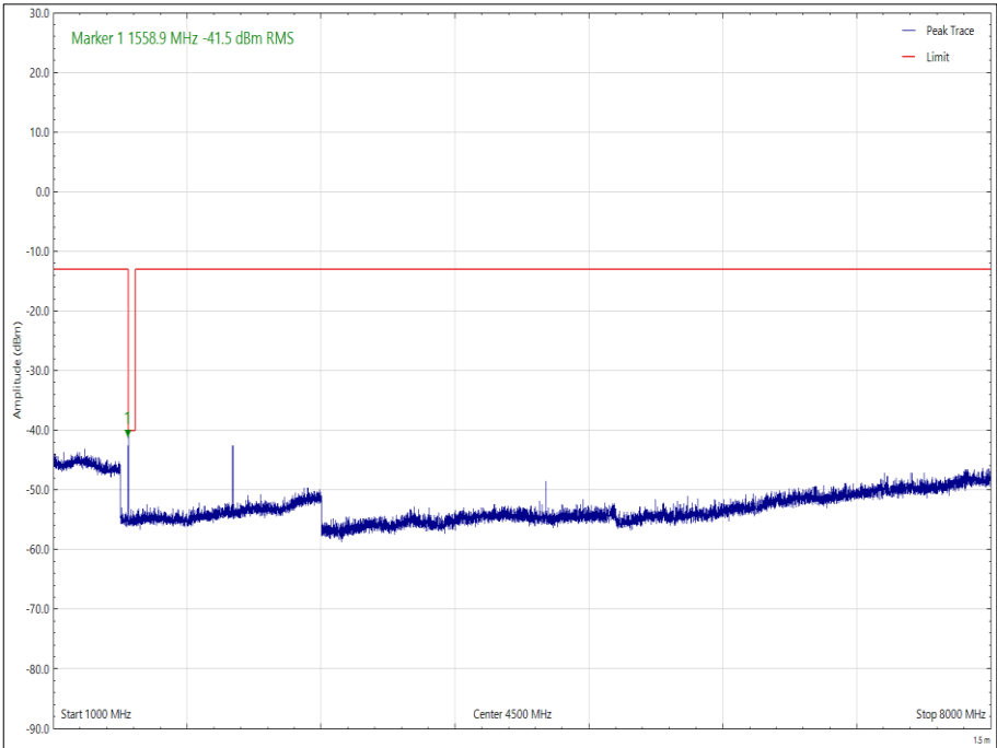
Figure 24 - 779.5 MHz - 1 GHz to 8 GHz, Horizontal, Orientation Y, Bottom Channel
