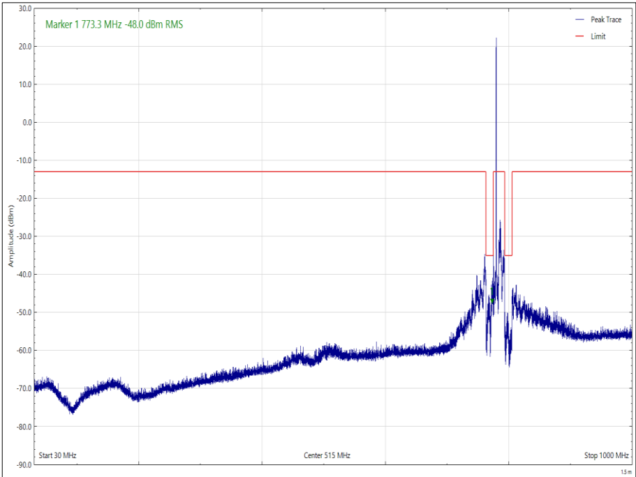
Figure 19 - 779.5 MHz - 30 MHz to 1 GHz, Horizontal, Orientation X, Bottom Channel
