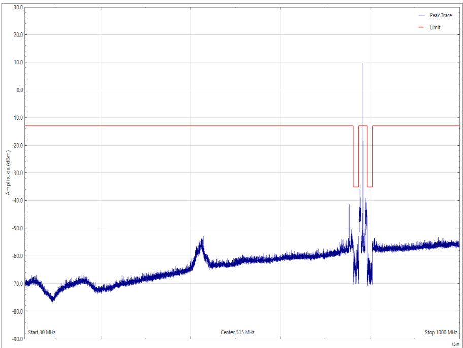
Figure 35 - 784.5 MHz - 30 MHz to 1 GHz, Horizontal, Orientation Y, Top Channel
