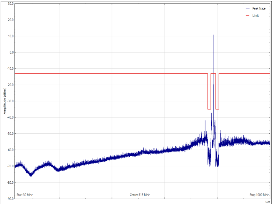
Figure 39 - 784.5 MHz - 30 MHz to 1 GHz, Horizontal, Orientation Z, Top Channel
