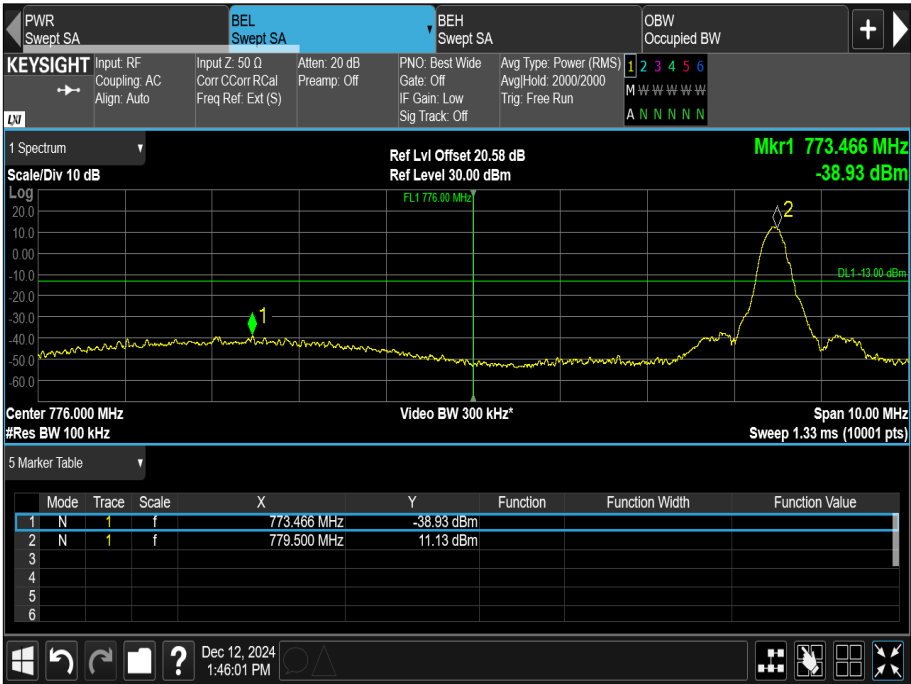
Figure 8 - Lower Band Edge, 779.5 MHz, Modulation: \pi/2 -BPSK, SCS: 15 kHz, Tone Number: 1, Start Sub-Carrier: 0
