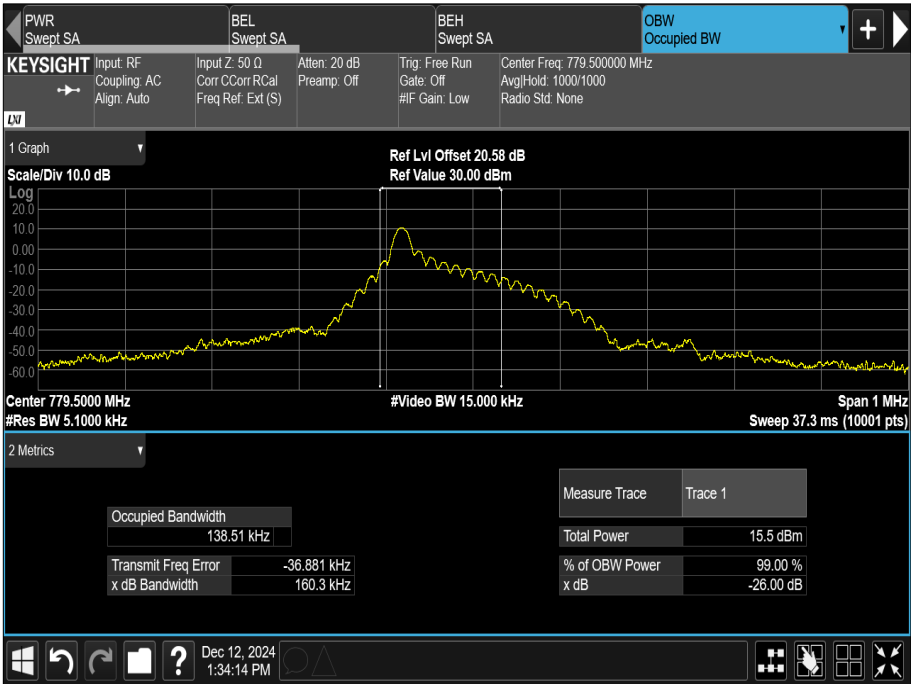
Figure 2 - Emission Bandwidth, 779.5 MHz, Modulation: \pi/4 -QPSK, SCS: 15 kHz, Tone Number: 1, Start Sub-Carrier: 0
