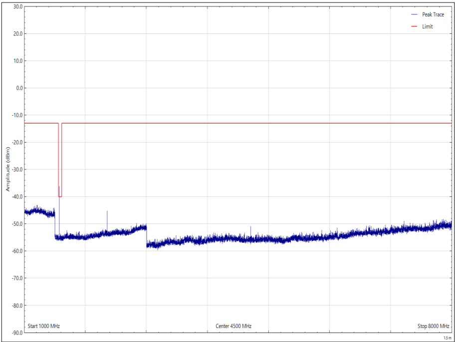
Figure 34 - 784.5 MHz - 1 GHz to 8 GHz, Vertical, Orientation X, Top Channel
