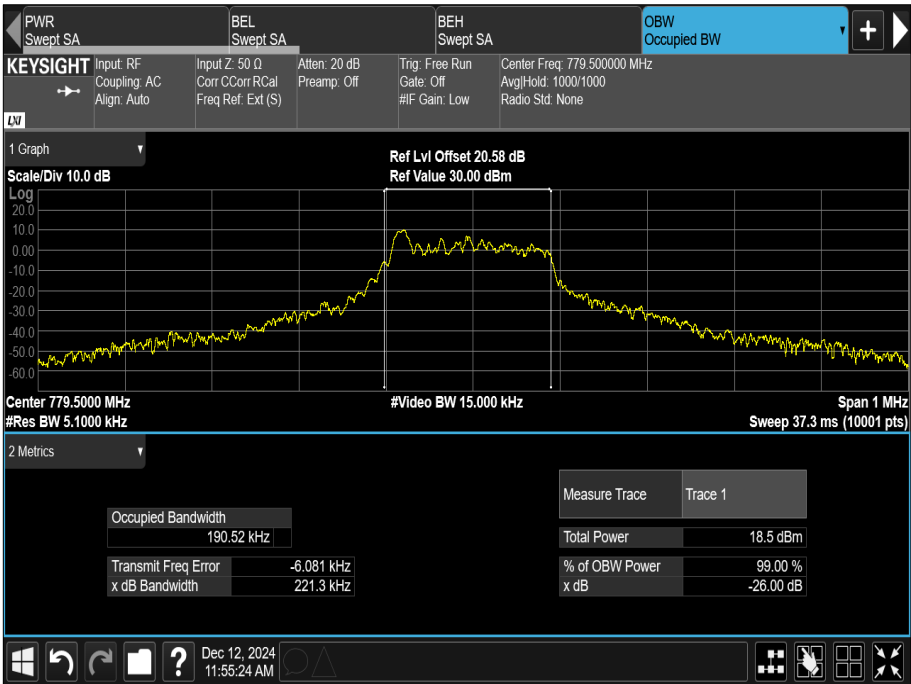
Figure 3 - Emission Bandwidth, 779.5 MHz, Modulation: QPSK, SCS: 15 kHz, Tone Number: 12, Start Sub-Carrier: 0
