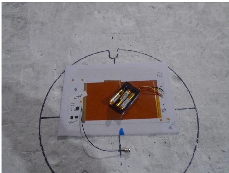
Figure 47 – EUT Orientation, Z Plane
