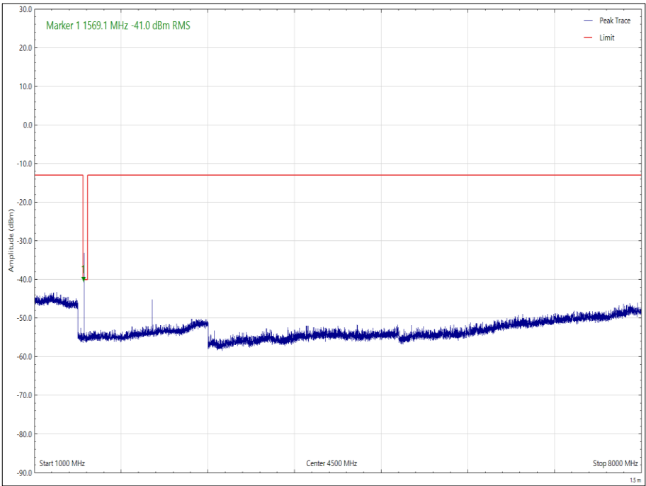
Figure 36 - 784.5 MHz - 1 GHz to 8 GHz, Horizontal, Orientation Y, Top Channel
