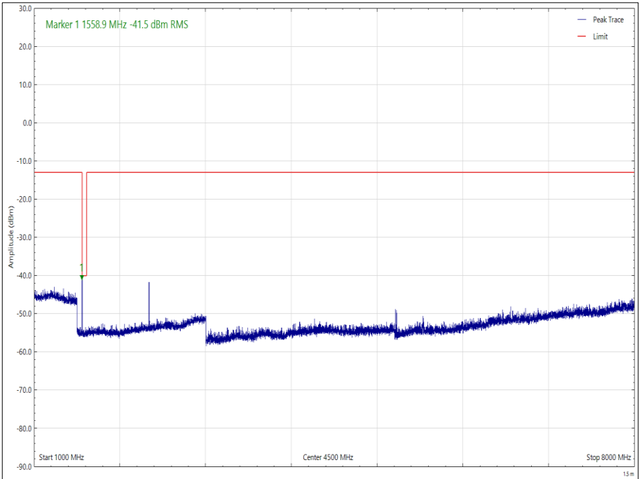
Figure 28 - 779.5 MHz - 1 GHz to 8 GHz, Horizontal, Orientation Z, Bottom Channel
