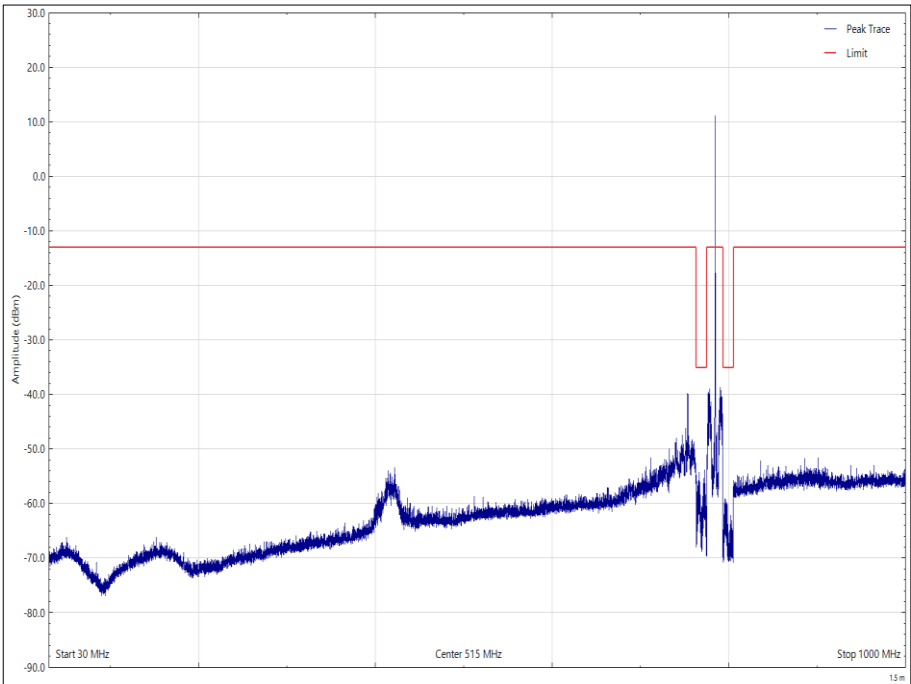
Figure 25 - 779.5 MHz - 30 MHz to 1 GHz, Vertical, Orientation Y, Bottom Channel
