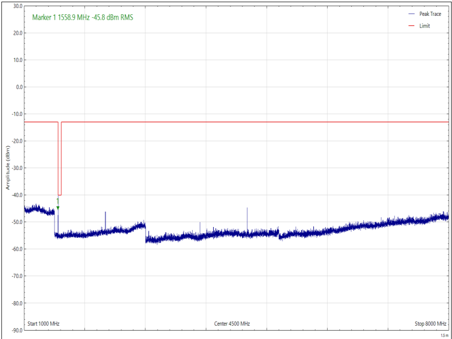
Figure 26 - 779.5 MHz - 1 GHz to 8 GHz, Vertical, Orientation Y, Bottom Channel
