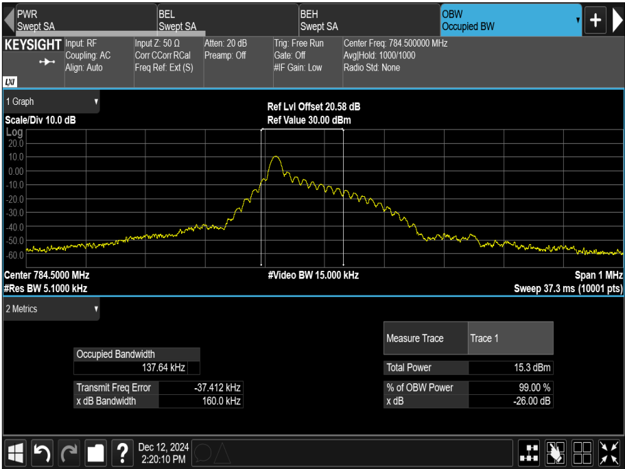
Figure 5 - Emission Bandwidth, 784.5 MHz, Modulation: \pi/4 -QPSK, SCS: 15 kHz, Tone Number: 1, Start Sub-Carrier: 0
