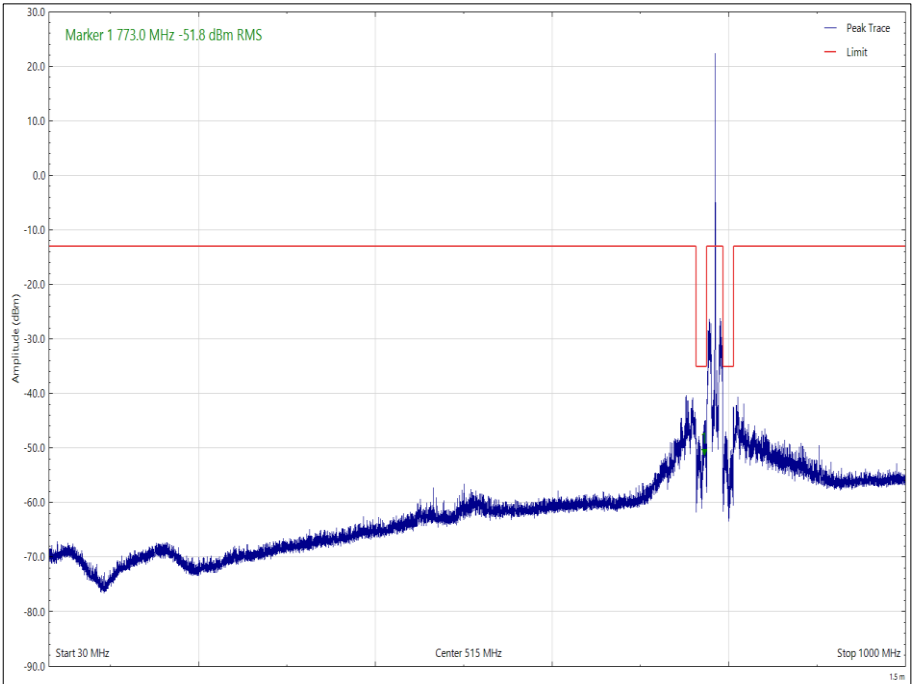
Figure 31 - 784.5 MHz - 30 MHz to 1 GHz, Horizontal, Orientation X, Top Channel
