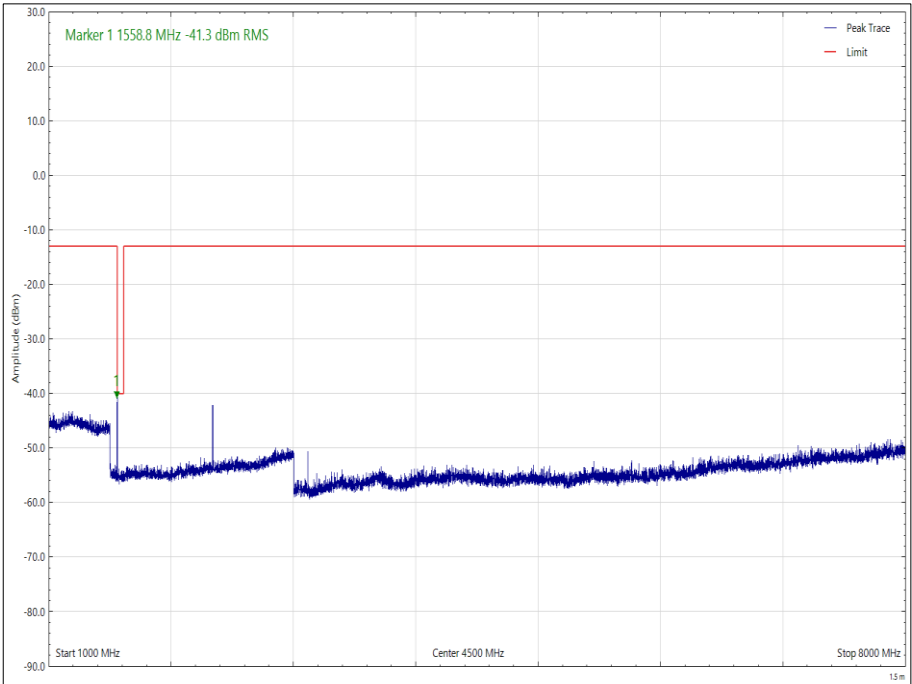
Figure 22 - 779.5 MHz - 1 GHz to 8 GHz, Vertical, Orientation X, Bottom Channel
