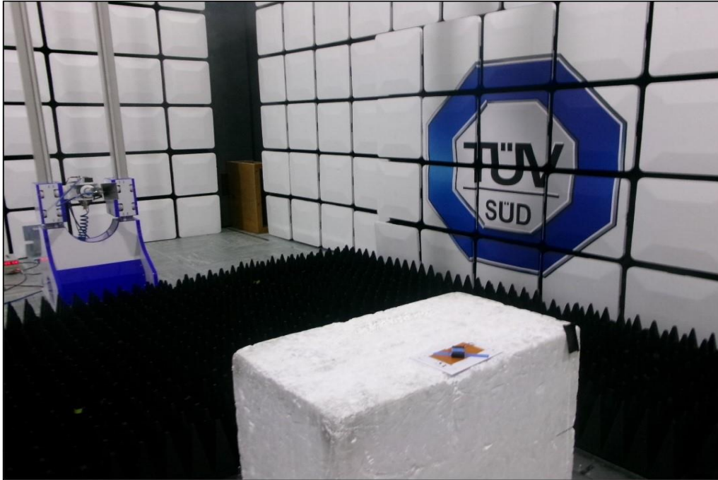
Figure 3 – Radiated Emissions – 8 GHz to 18 GHz
