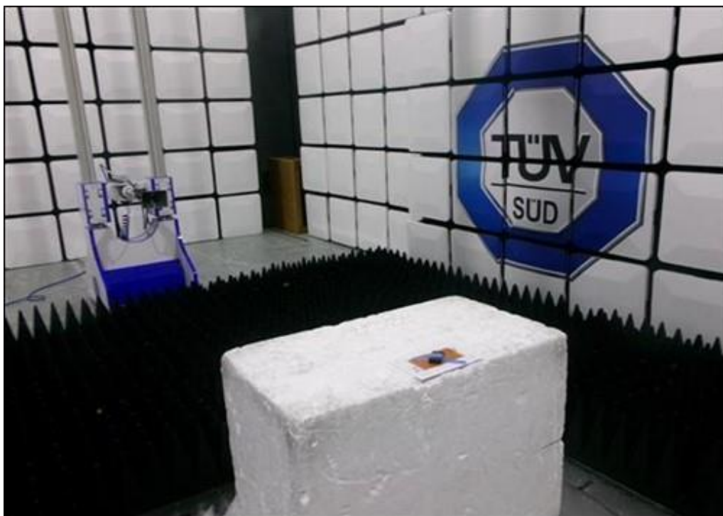
Figure 2 – Radiated Emissions – 1 GHz to 8 GHz
