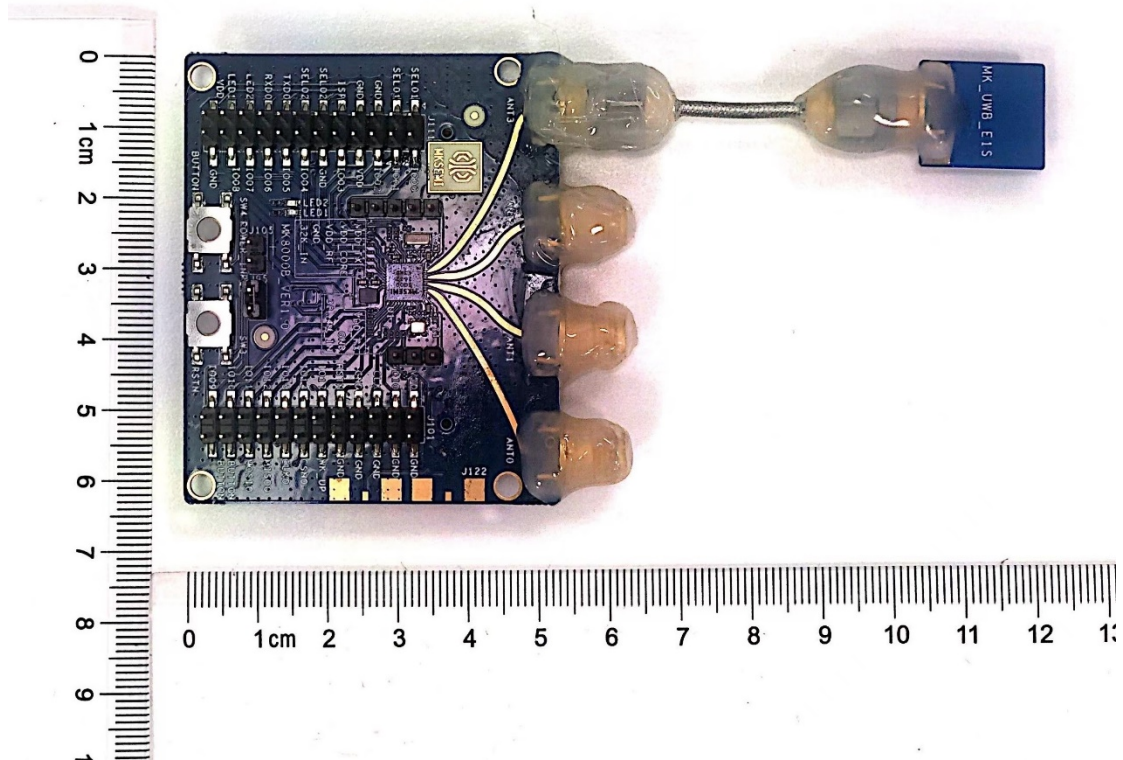
Antenna Mode 1 Front
