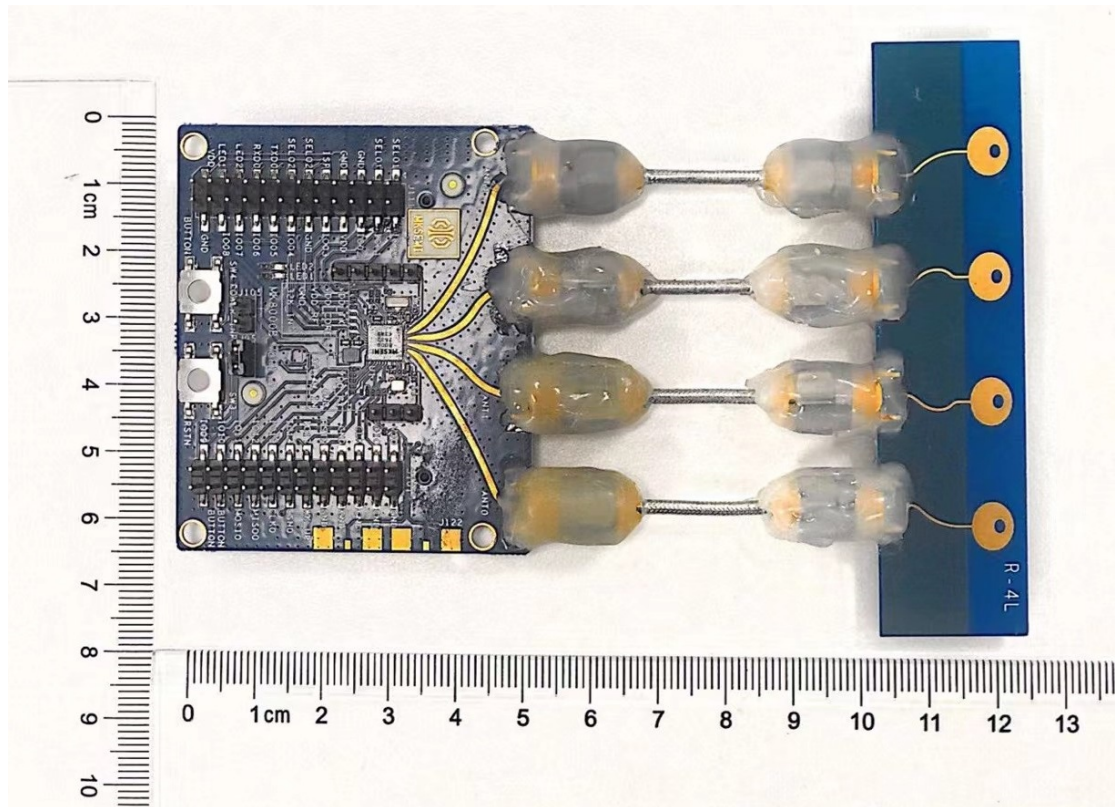
Antenna Mode 2 Front
