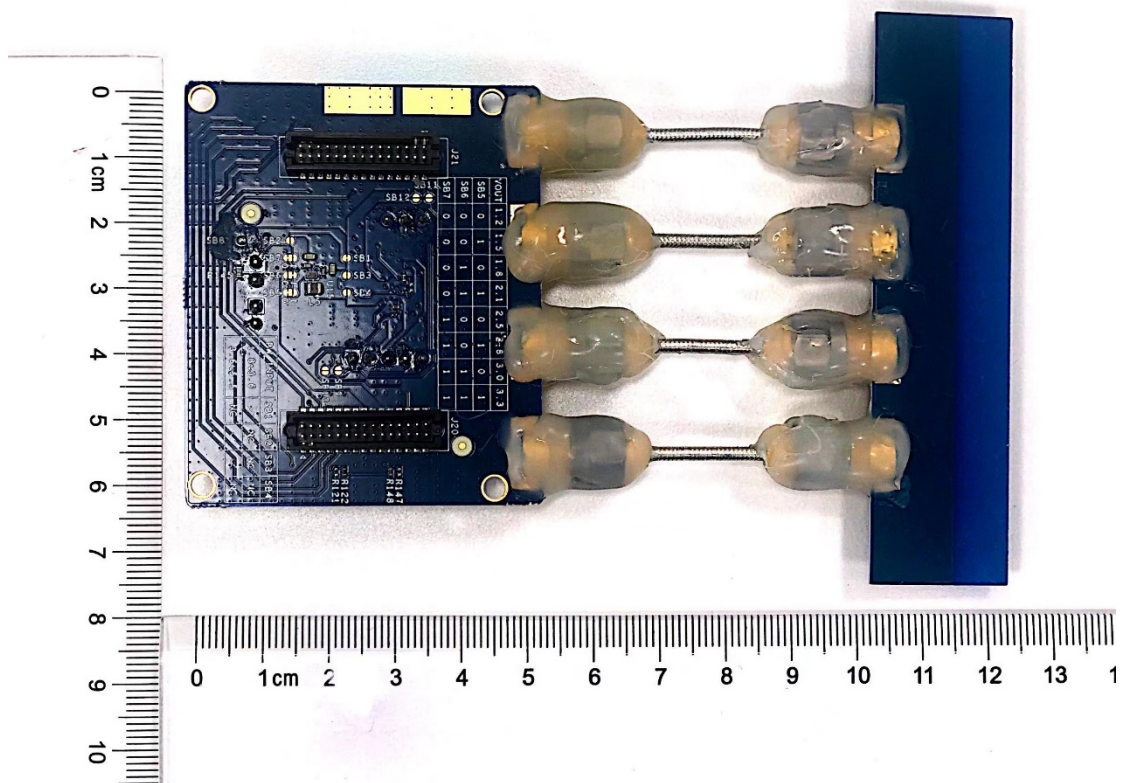
Antenna Mode 2 Back
