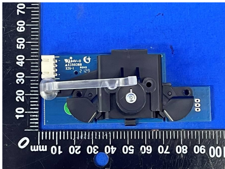
PCBA view of charging dock
