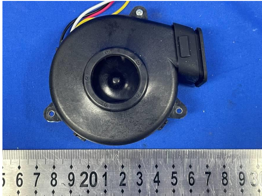
Suction motor view of robotic vacuum cleaner
