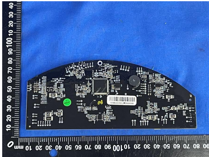
PCBA view of robotic vacuum cleaner
