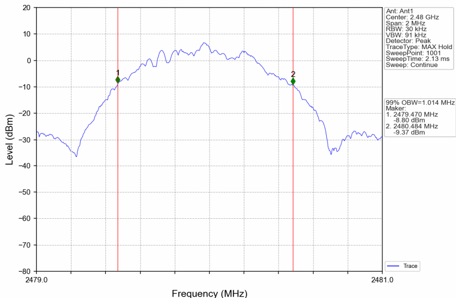
1M_HCH_2480MHz_Ant1_NTNV
