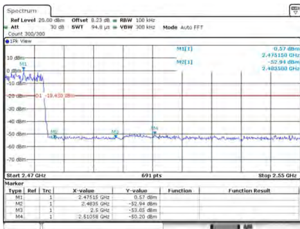
3DH5(2480)-Hopping on
