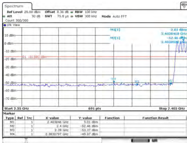
DH5(2402)-Hopping on
