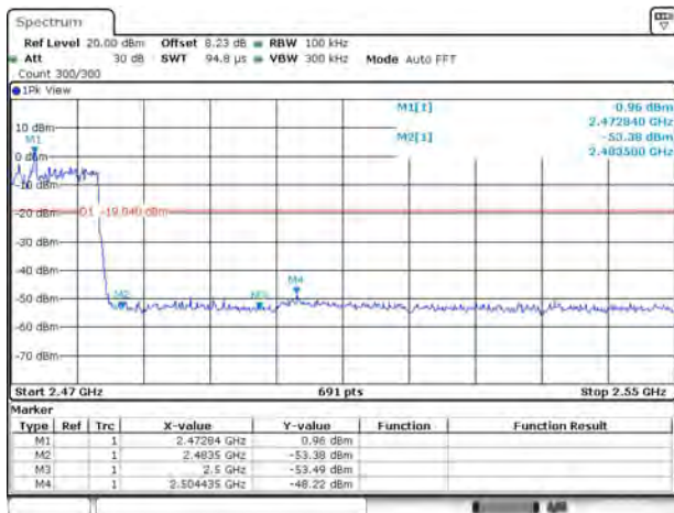
2DH5(2480)-Hopping on
