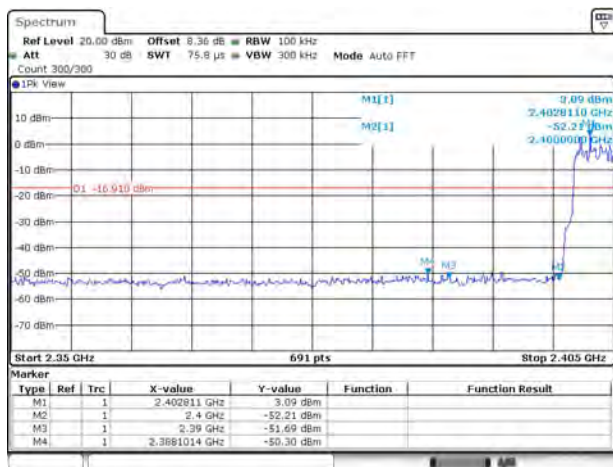
3DH5(2402)-Hopping on
