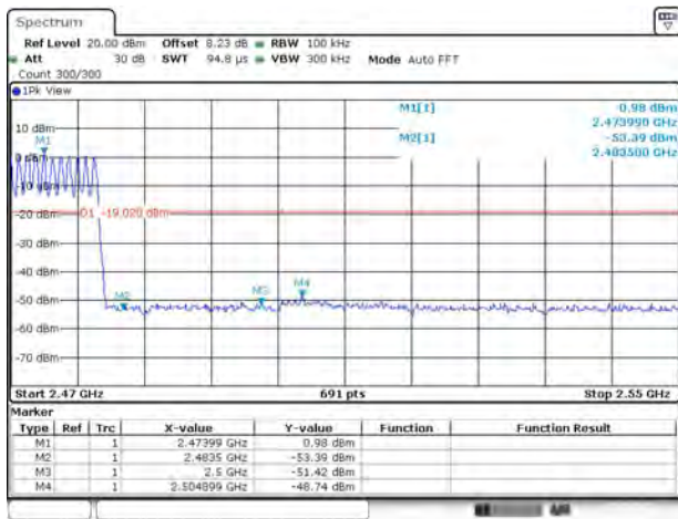
DH5(2480)-Hopping on
