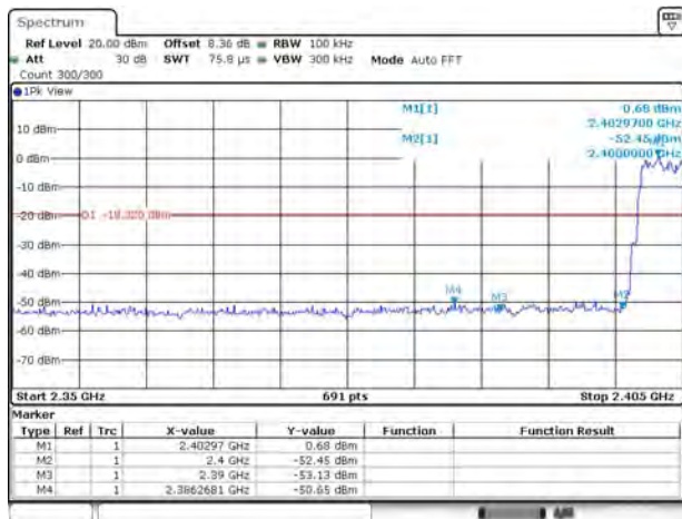
2DH5(2402)-Hopping on
