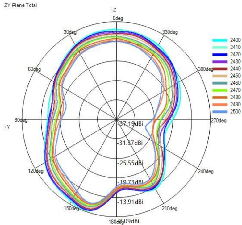
(2) Y-Z Plane(unit:dBi):
