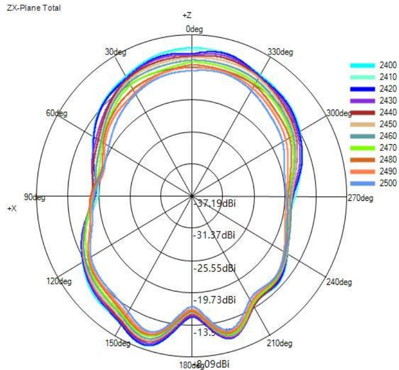
(1) X-Z Plane(unit:dBi):
