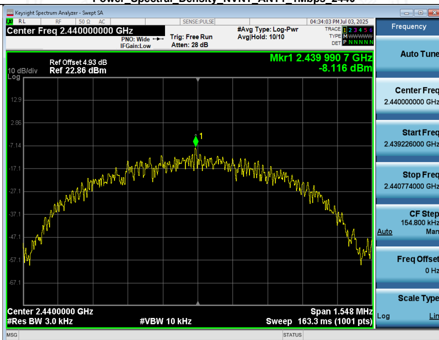
Power Spectral Density_NVNT_ANT1_1Mbps_2440
