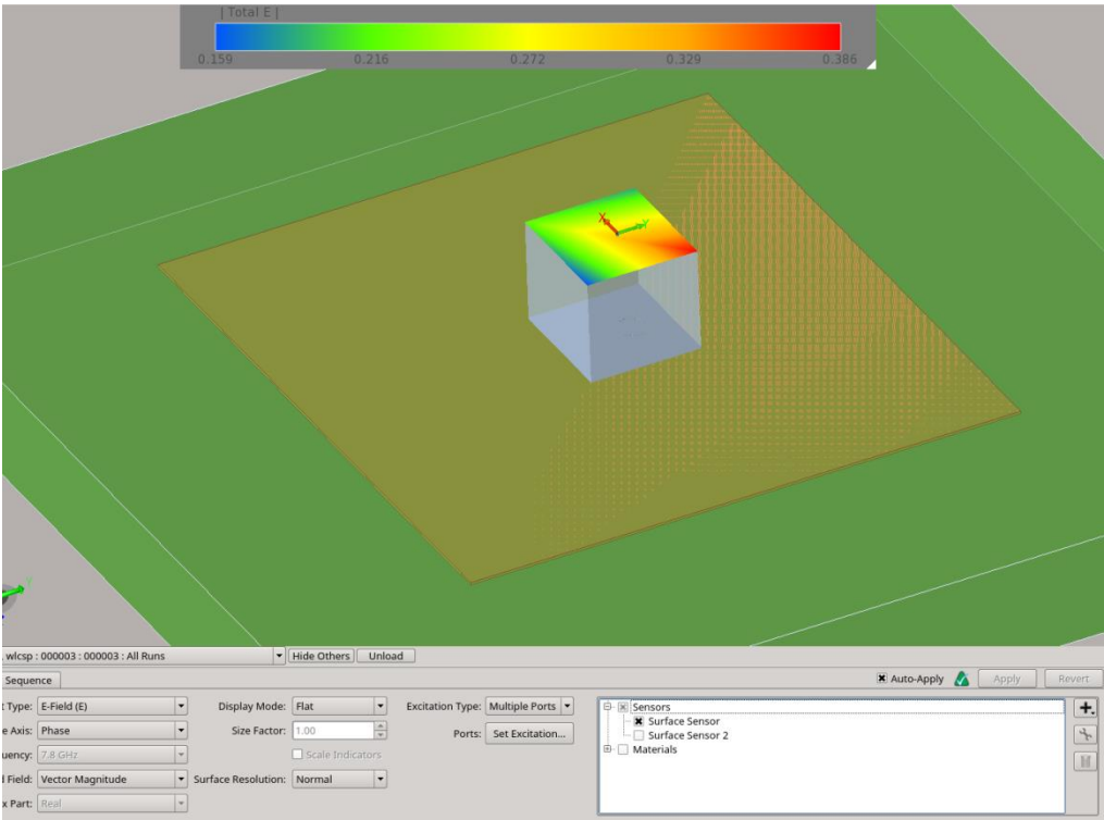
Figure 17 Surface E-Field Magnitude at top of the chip for the LT102XK
