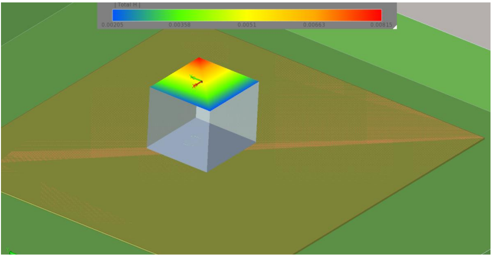
Figure 18 Surface H-Field Magnitude at top of the chip (BEOL side) for the LT102XK
