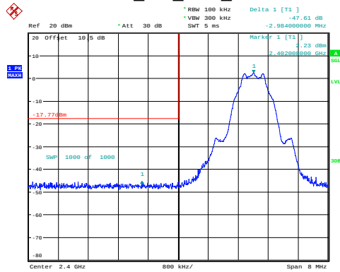
BLE_1M_Low_Channel
