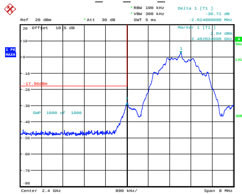
BLE_2M_Low_Channel
