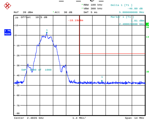
BLE_2M_High_Channel
