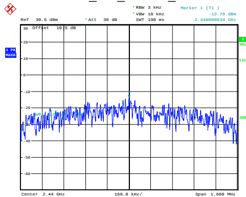
BLE_2M_Middle_Channel
