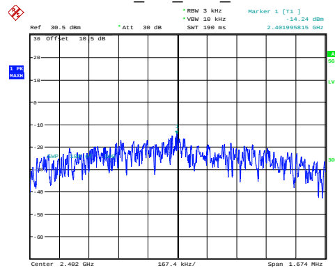
BLE_2M_Low_Channel
