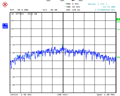
BLE_1M_High_Channel
