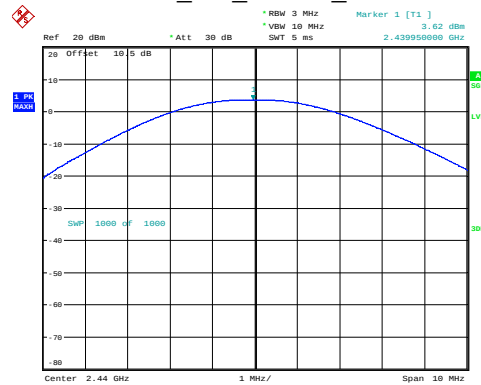
BLE_1M_Middle_Channel
