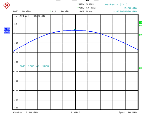
BLE_2M_High_Channel
