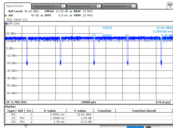
n20_5785MHz_Chain 0
