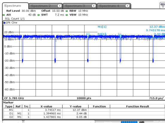
a_5785MHz_Chain 0
