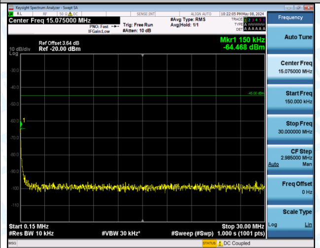
Band7_15MHz_QPSK_21375_1RB#74_1000~20000_1000~20000
