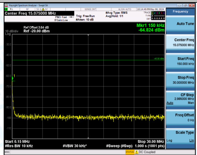
Band7_15MHz_QPSK_20825_1RB#74_1000~20000_1000~20000
