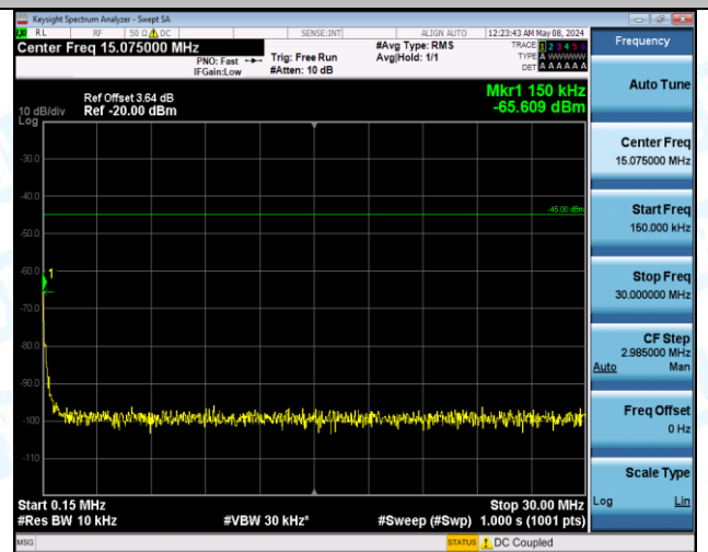
Band7_5MHz_16QAM_21100_25RB#0_1000~20000_1000~20000
