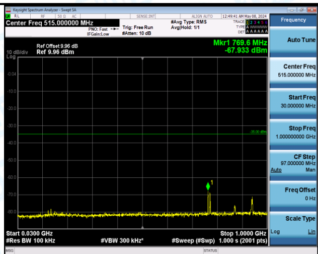
Band7_10MHz_QPSK_20800_1RB#49_20000~27000_20000~27000
