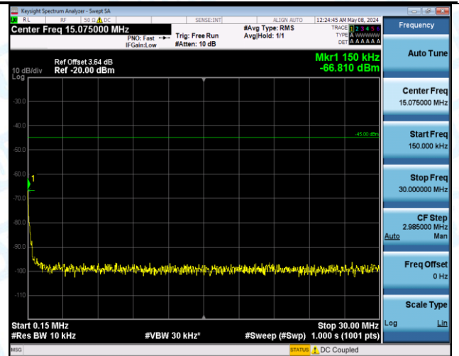
Band7_5MHz_QPSK_21425_1RB#0_1000~20000_1000~20000
