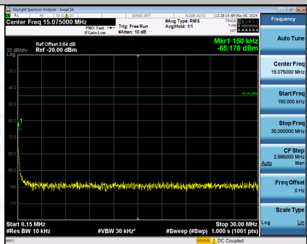
Band7_5MHz_QPSK_21425_25RB#0_1000-20000_1000-20000
