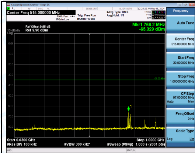
Band7_5MHz_QPSK_21425_25RB#0_20000~27000_20000~27000
