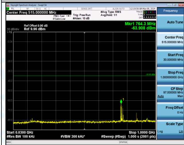
Band7_5MHz_16QAM_21100_1RB#0_20000~27000_20000~27000
