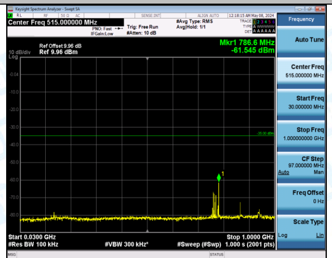
Band7_5MHz_QPSK_21100_1RB#0_20000~27000_20000~27000
