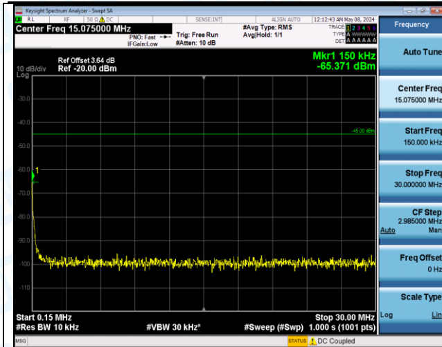
Band7_5MHz_QPSK_20775_1RB#24_1000-20000_1000-20000
