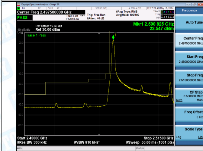
Band7_15MHz_QPSK_20825_75RB#0
